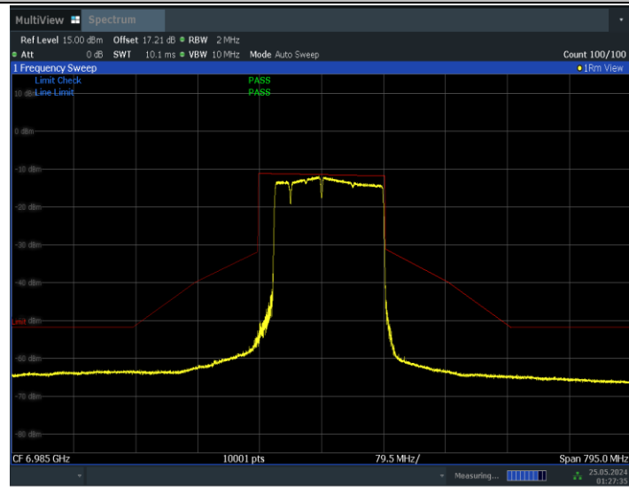
11BE160MIMO_Ant1_6985_996+484+242_Non-OFDMA_1
