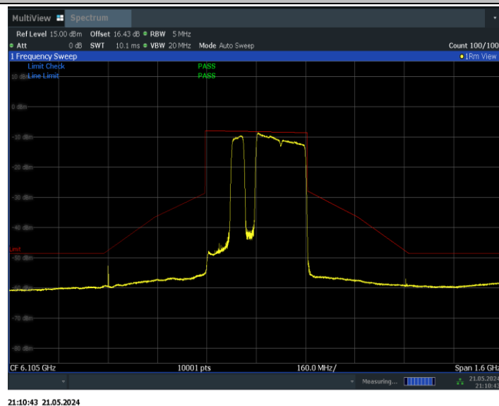
11BE320MIMO_Ant1_6105_2*996+484_Non-OFDMA_8
