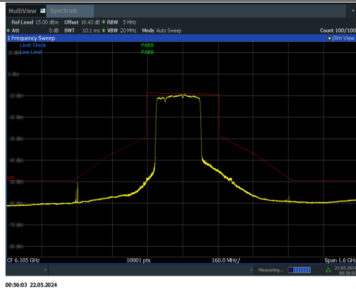
11BE320MIMO_Ant1_6105_2*996+484_Non-OFDMA_2
