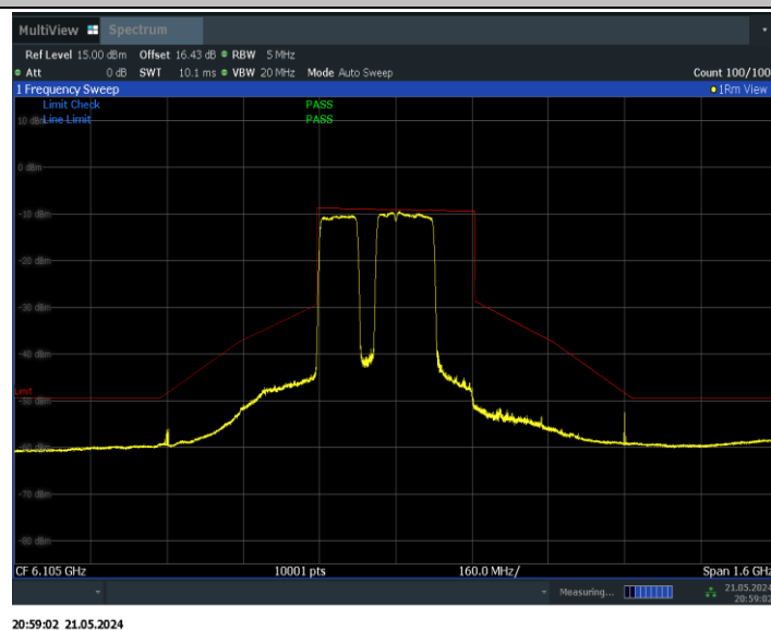
11BE320MIMO_Ant1_6105_2*996+484_Non-OFDMA_3
