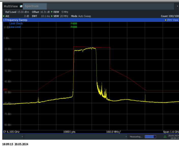
11BE320MIMO_Ant0_6105_2*996+484_Non-OFDMA_7
