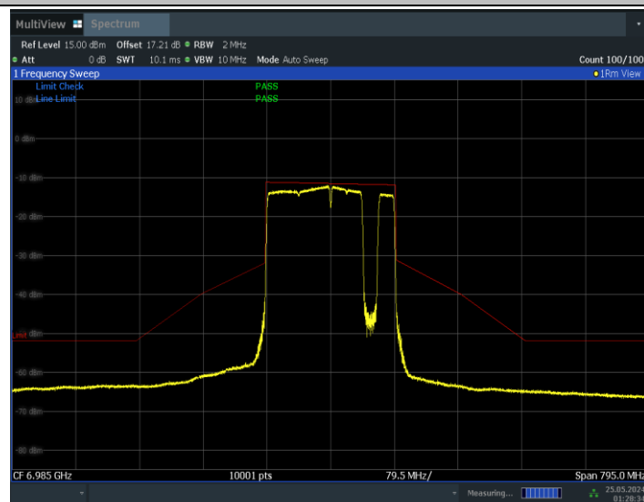
11BE160MIMO_Ant1_6985_996+484+242_Non-OFDMA_7
