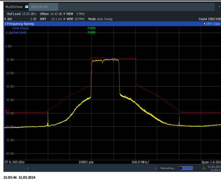
11BE320MIMO_Ant1_6105_2*996+484_Non-OFDMA_7
