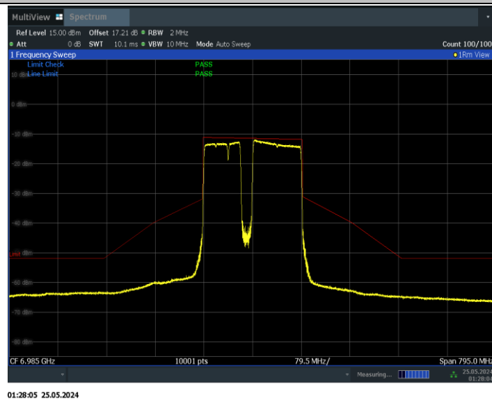
11BE160MIMO_Ant1_6985_996+484+242_Non-OFDMA_5
