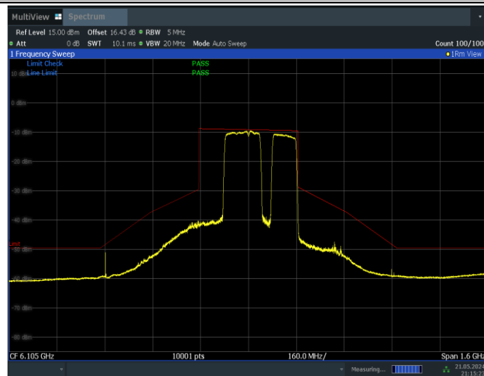
11BE320MIMO_Ant1_6105_2*996+484_Non-OFDMA_10
