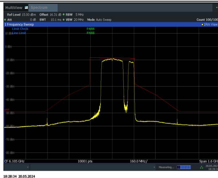
11BE320MIMO_Ant0_6105_2*996+484_Non-OFDMA_12
