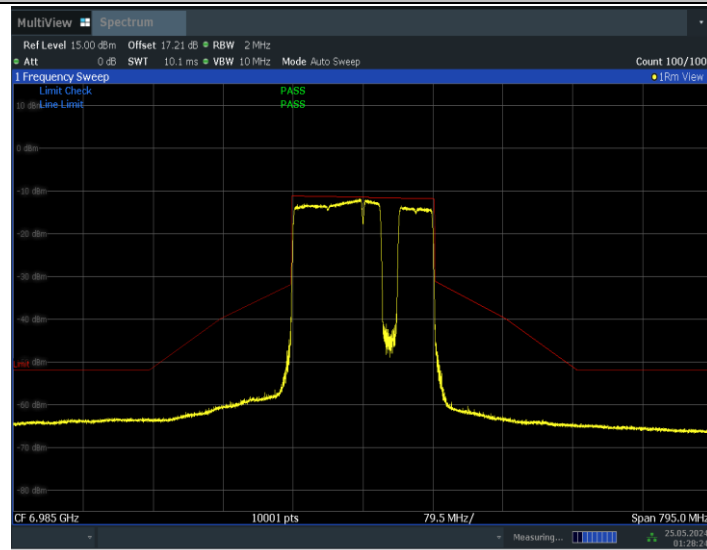
11BE160MIMO_Ant1_6985_996+484+242_Non-OFDMA_6
