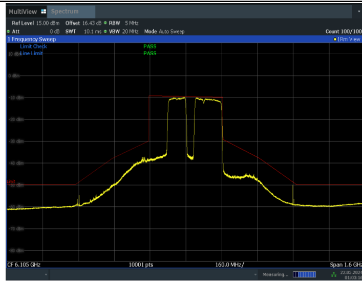
11BE320MIMO_Ant1_6105_2*996+484_Non-OFDMA_9
