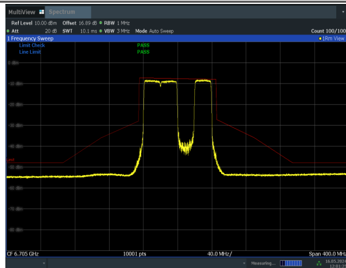
11BE80MIMO_Ant1_6705_484+242_Non-OFDMA_3
