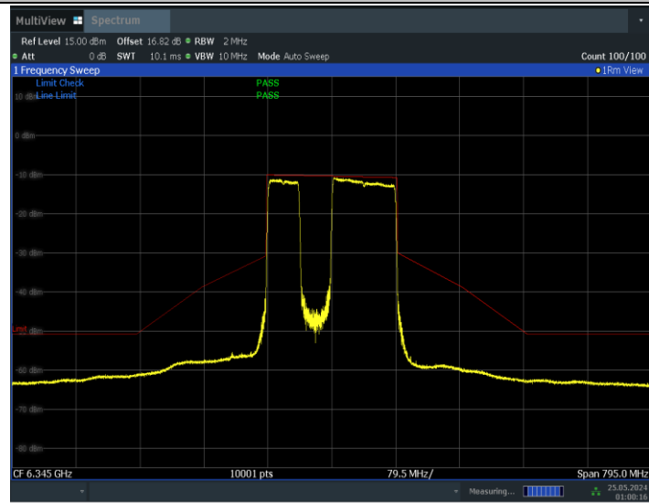
11BE160MIMO_Ant0_6345_996+484_Non-OFDMA_3
