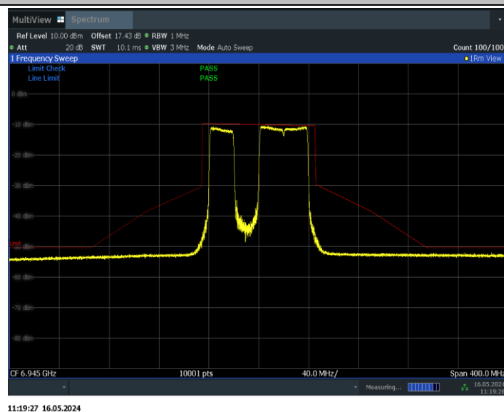
11BE80MIMO_Ant1_6945_484+242_Non-OFDMA_2
