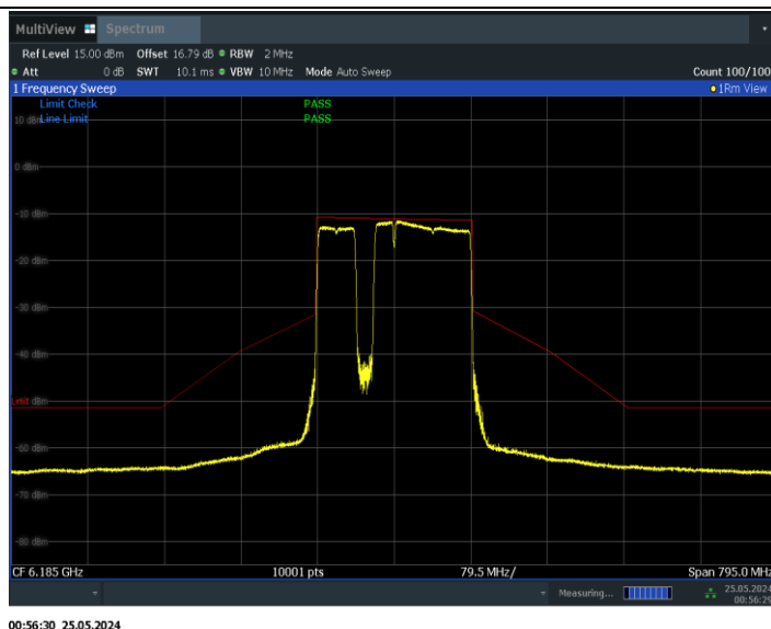
11BE160MIMO_Ant1_6185_996+484+242_Non-OFDMA_4
