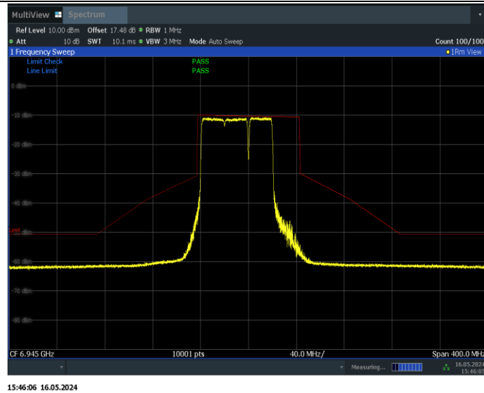
11BE80MIMO_Ant1_6945_484+242_Non-OFDMA_1
