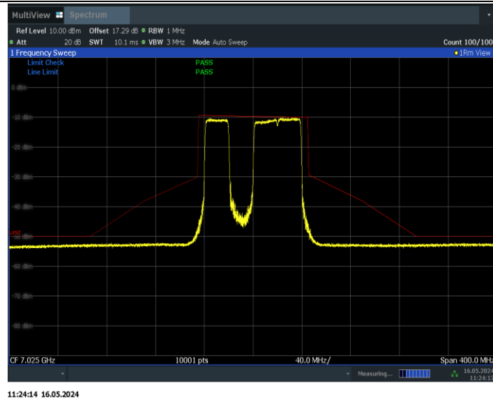
11BE80MIMO_Ant1_7025_484+242_Non-OFDMA_3
