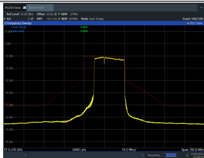
11BE160MIMO_Ant0_6345_996+484_Non-OFDMA_4
