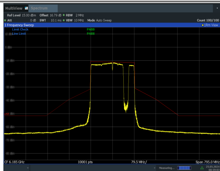
11BE160MIMO_Ant1_6185_996+484+242_Non-OFDMA_7
