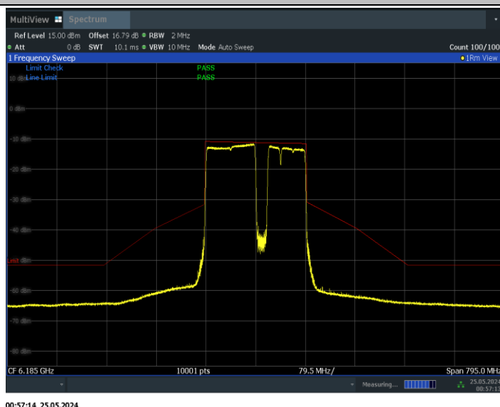
11BE160MIMO_Ant1_6185_996+484+242_Non-OFDMA_5
