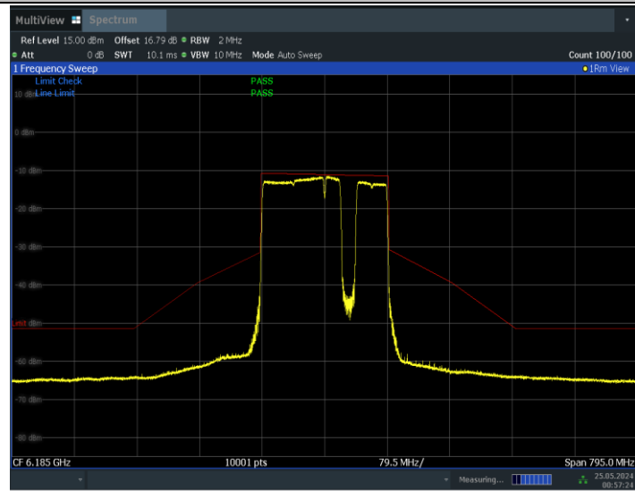
11BE160MIMO_Ant1_6185_996+484+242_Non-OFDMA_6
