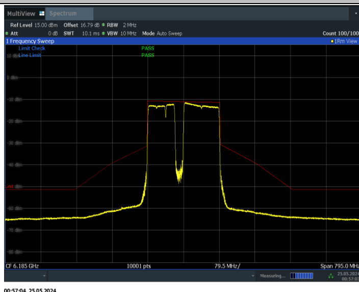
11BE160MIMO_Ant1_6185_996+484+242_Non-OFDMA_5
