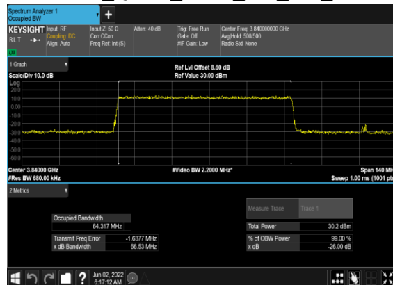
B5_N77(70M)_DFT-s- OFDM_QPSK_Outer_Full_Mid_CH
