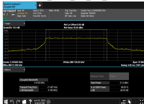
B5_N7(5M)_CP-OFDM_256 QAM_Outer_Full_Mid_CH
