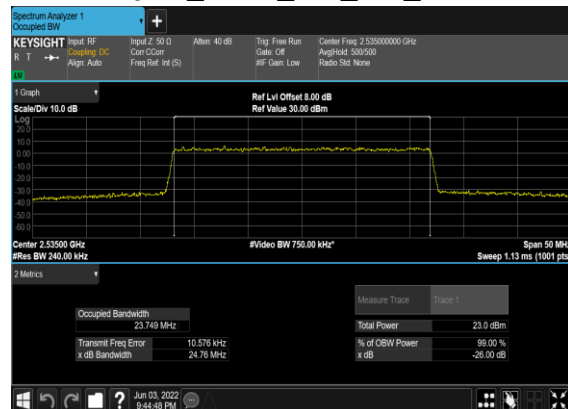
B5_N7(25M)_CP-OFDM_256 QAM_Outer_Full_Mid_CH
