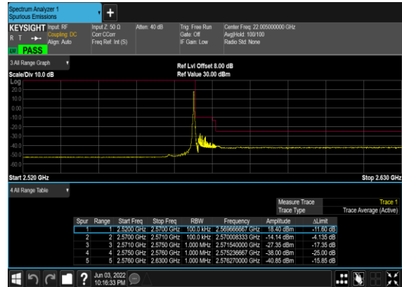
B5_N7(5M)_DFT-s- OFDM_QPSK_Edge_1RB_Right_High_CH
