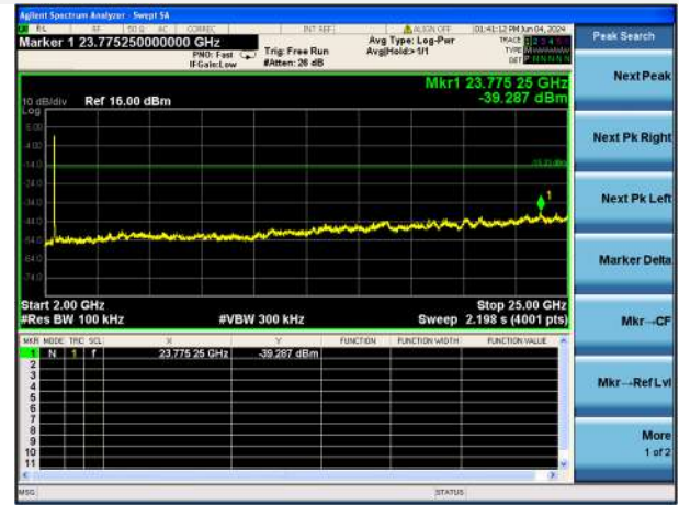
802.11n-20 MHz CHANNEL 1, SPURIOUS 2 GHz ~ 25 GHz
