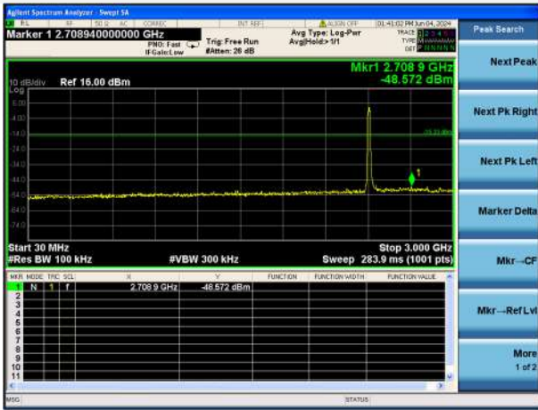
802.11n-20 MHz CHANNEL 1, SPURIOUS 30 MHz ~ 3 GHz
