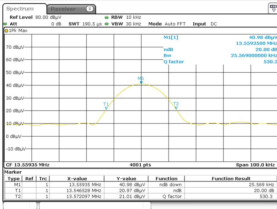
Emission Bandwidth
