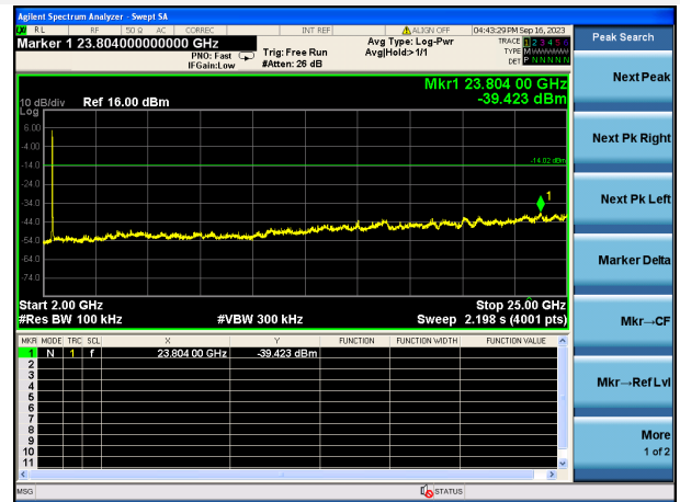
802.11n-20 MHz CHANNEL 1, SPURIOUS 2 GHz ~ 25 GHz
