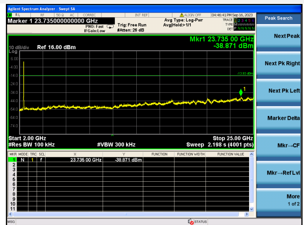
802.11n-20 MHz CHANNEL 6, SPURIOUS 2 GHz ~ 25 GHz
