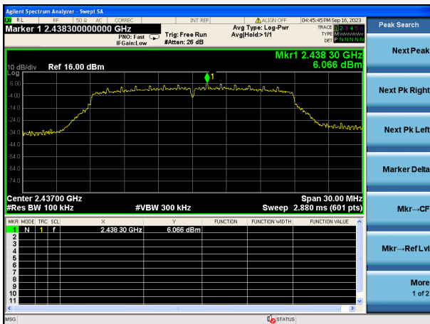
802.11n-20 MHz CHANNEL 6 CARRIER LEVEL
