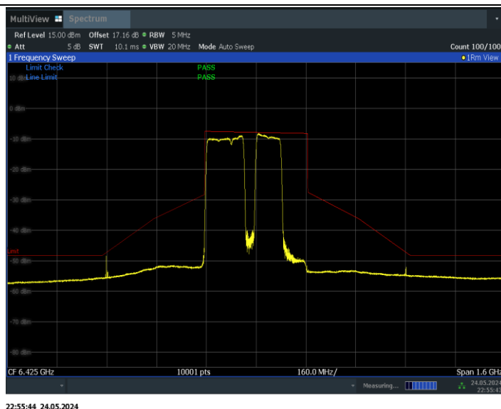
11BE320MIMO_Ant0_6425_2*996+484_Non-OFDMA_5
