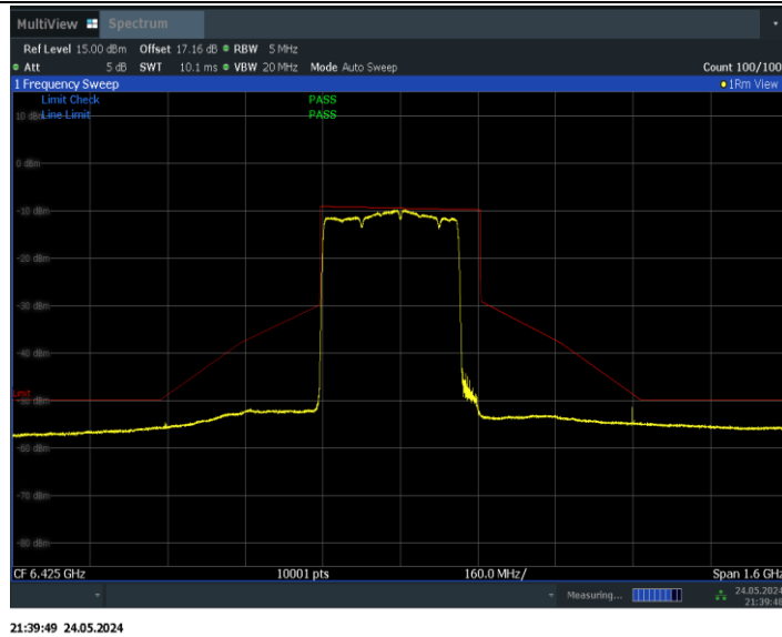
11BE320MIMO_Ant1_6425_2*996+484_Non-OFDMA_1
