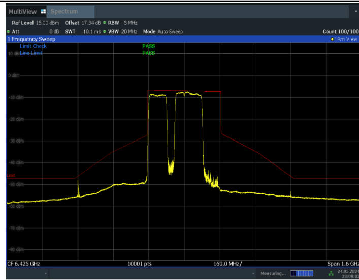
11BE320MIMO_Ant1_6425_2*996+484_Non-OFDMA_3
