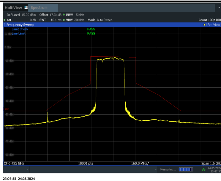
11BE320MIMO_Ant1_6425_2*996+484_Non-OFDMA_2
