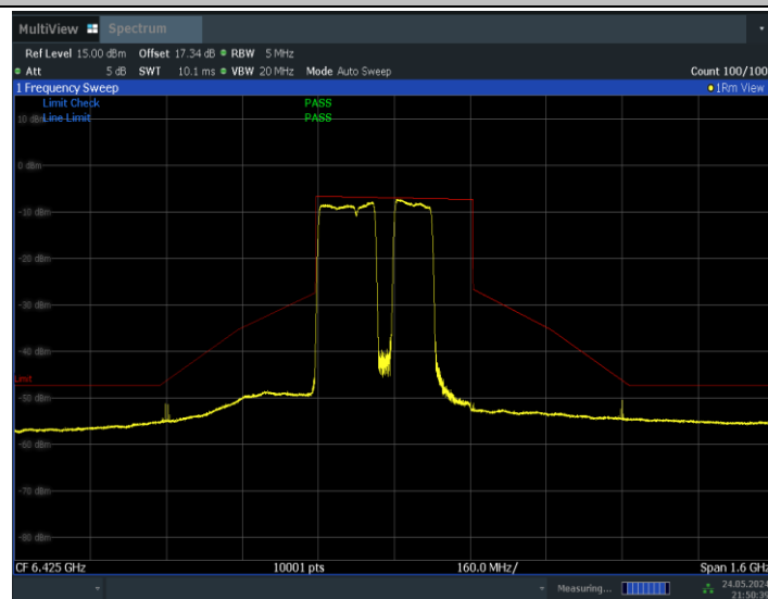
11BE320MIMO_Ant1_6425_2*996+484_Non-OFDMA_4
