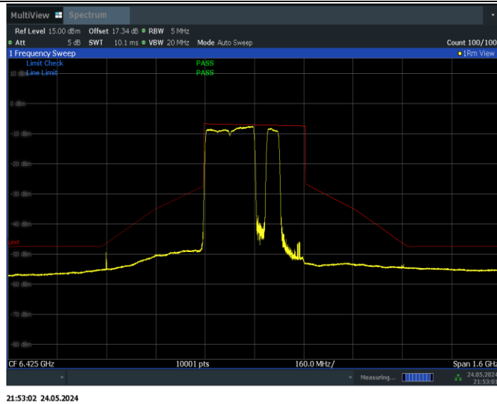
11BE320MIMO_Ant1_6425_2*996+484_Non-OFDMA_6
