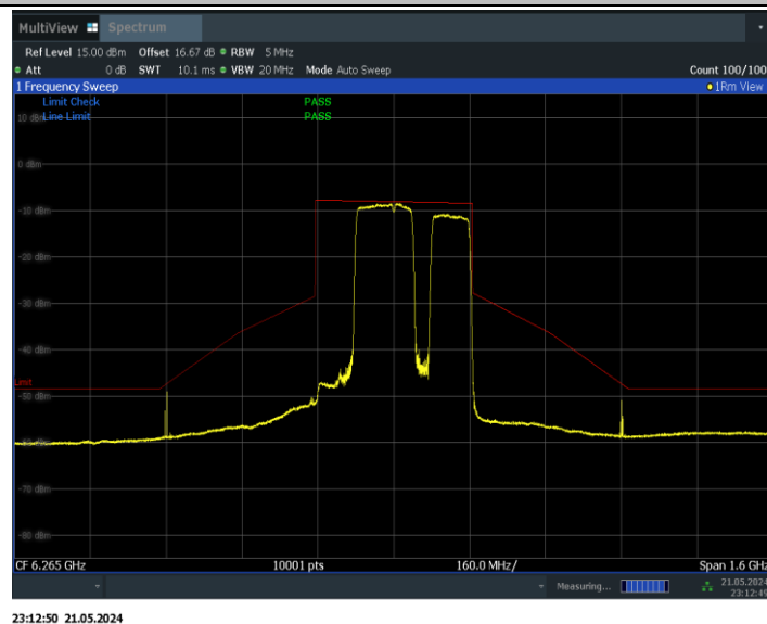
11BE320MIMO_Ant1_6265_2*996+484_Non-OFDMA_10
