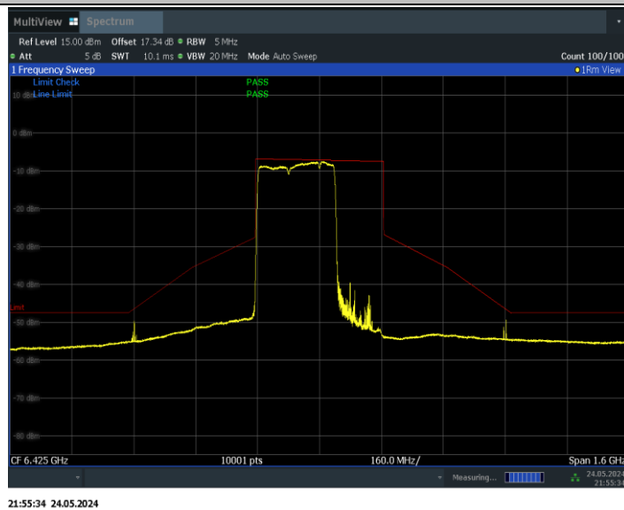
11BE320MIMO_Ant1_6425_2*996+484_Non-OFDMA_7
