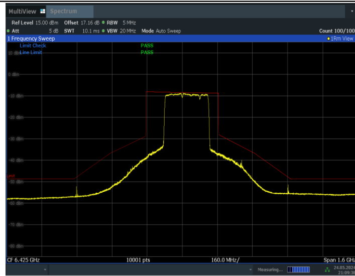
11BE320MIMO_Ant0_6425_2*996+484_Non-OFDMA_12
