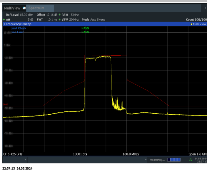
11BE320MIMO_Ant0_6425_2*996+484_Non-OFDMA_6
