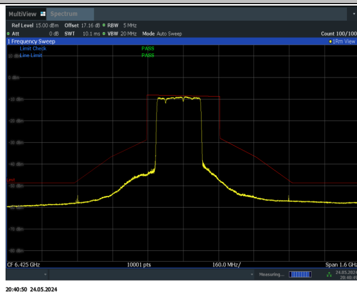
11BE320MIMO_Ant0_6425_2*996+484_Non-OFDMA_1
