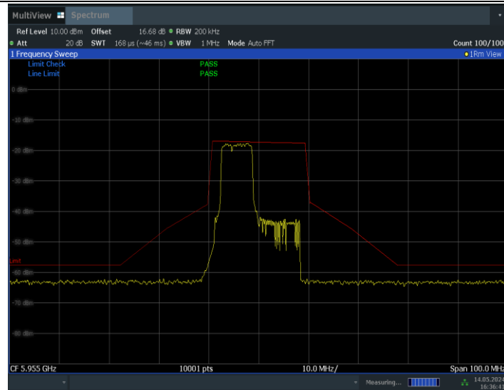
11BE20MIMO_Ant1_5955_106+26_OFDMA_1
