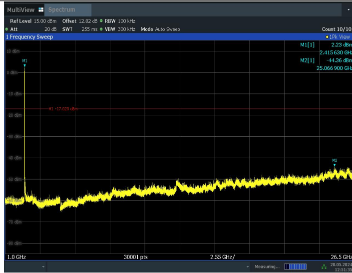
11BE20MIMO_Ant1_2412_52+26_OFDMA_1_0~Reference
