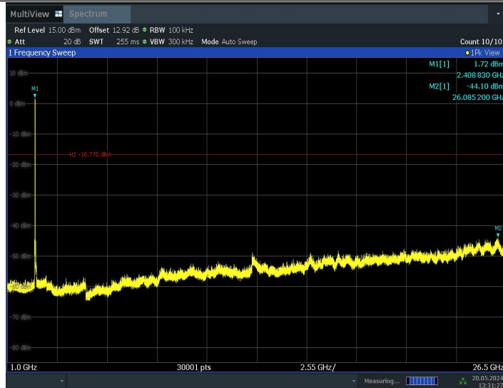
11BE20MIMO_Ant1_2412_106+26_OFDMA_1_1000~26500
