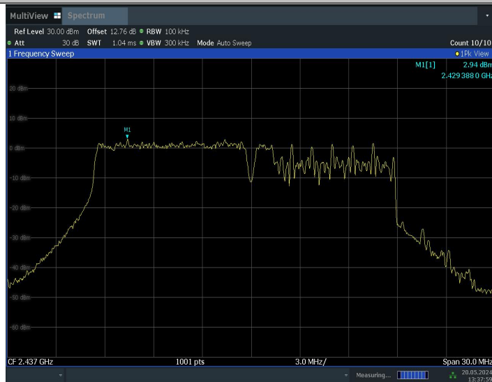
11BE20MIMO_Ant0_2437_106+26_OFDMA_1_0~Reference
