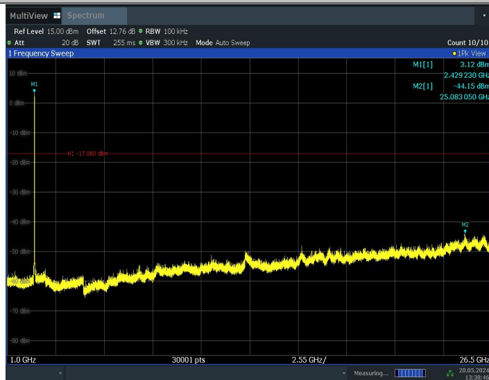
11BE20MIMO_Ant0_2437_106+26_OFDMA_1_1000~26500
