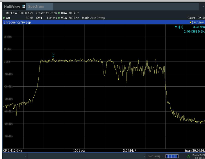
11BE20MIMO_Ant1_2412_106+26_OFDMA_1_0~Reference
