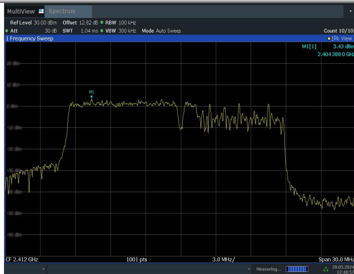
11BE20MIMO_Ant0_2412_106+26_OFDMA_1_0~Reference
