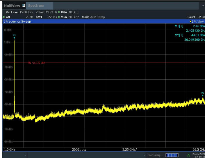
11BE20MIMO_Ant0_2412_106+26_OFDMA_1_1000~26500
