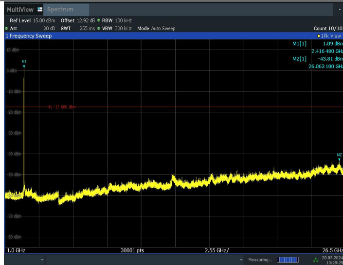
11BE20MIMO_Ant1_2412_106+26_OFDMA_1_0~Reference
