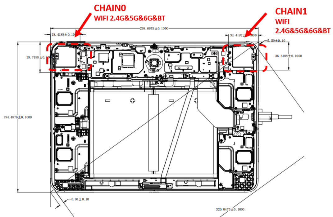
Picture 7 Antenna location
