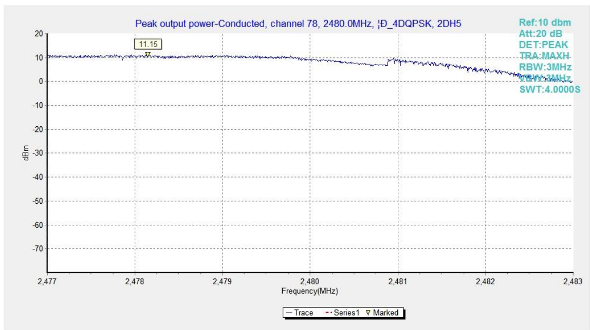
Fig.15. Peak Output Power -Conducted: \pi/4 DQPSK, Channel 78, ANT1
