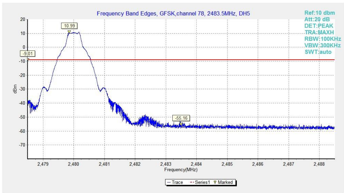
Fig.21. Frequency Band Edges: GFSK, Channel 78, Hopping Off
