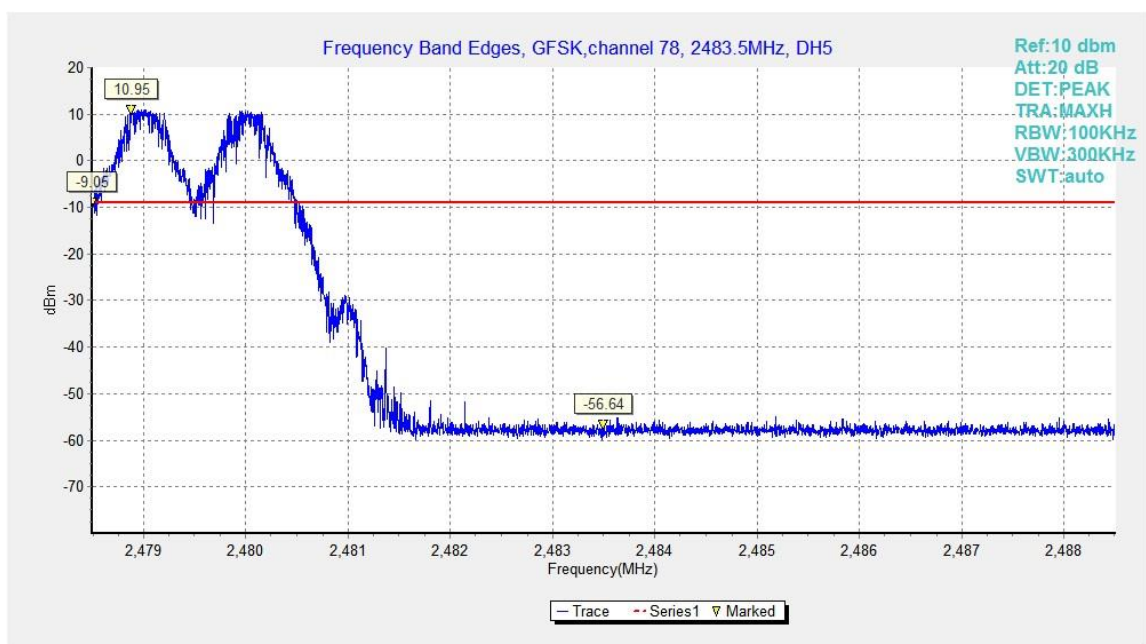
Fig.22. Frequency Band Edges: GFSK, Channel 78, Hopping On
