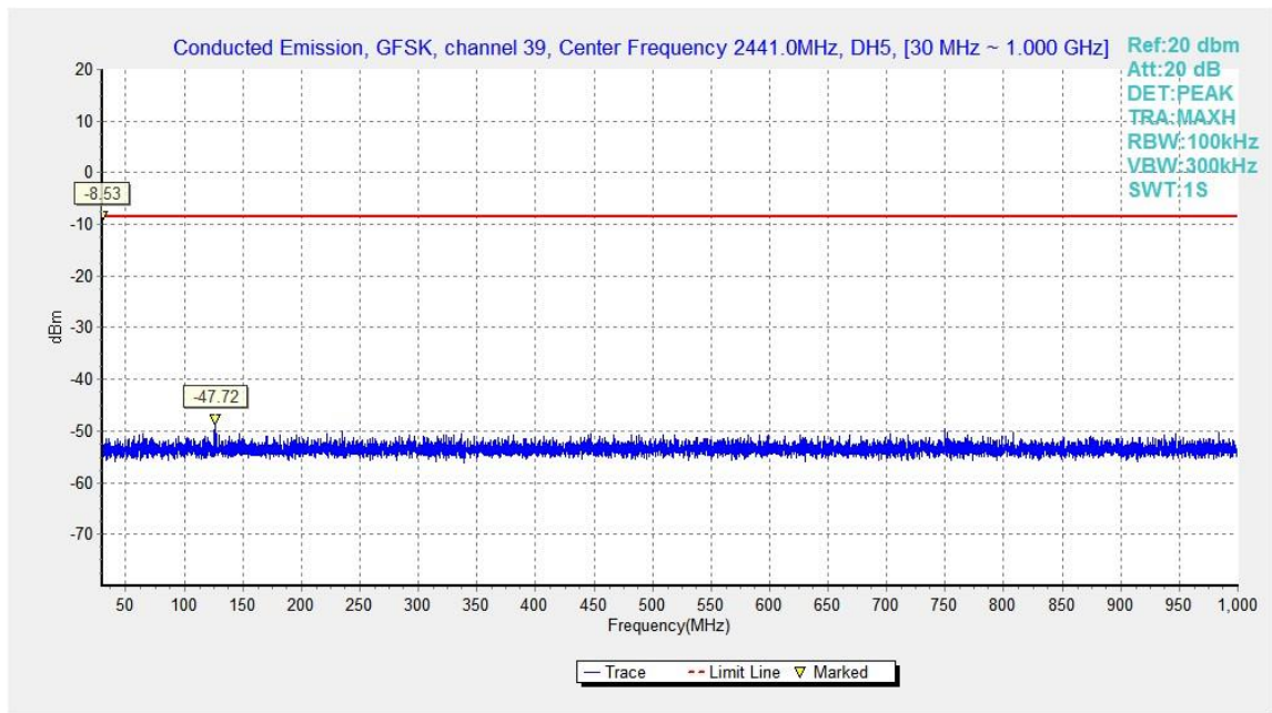
Fig.37. Conducted spurious emission: GFSK, Channel 39, 30MHz - 1GHz
