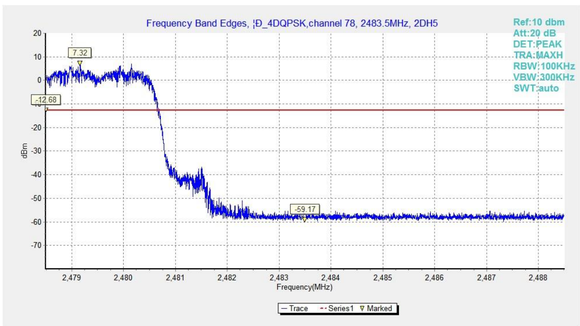
Fig.26. Frequency Band Edges: \pi/4 DQPSK, Channel 78, Hopping On
