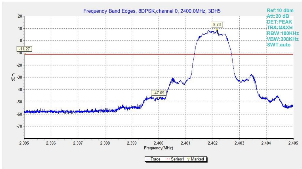
Fig.27. Frequency Band Edges: 8DPSK, Channel 0, Hopping Off
