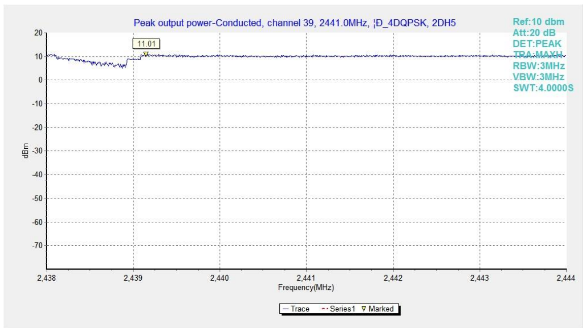
Fig.14. Peak Output Power -Conducted: \pi/4 DQPSK, Channel 39, ANT1
