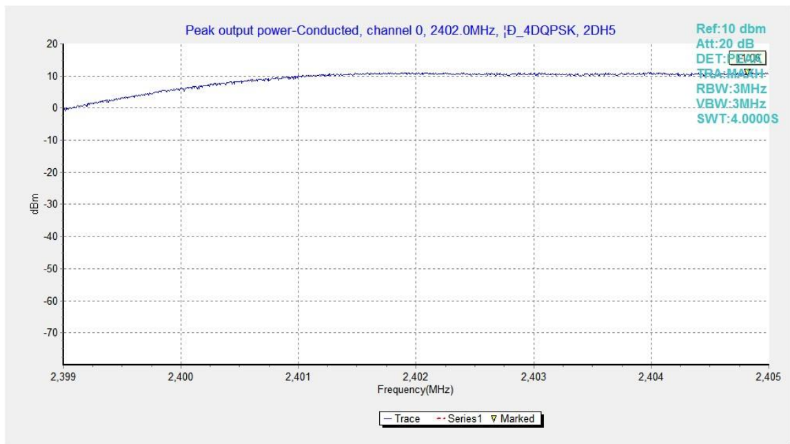
Fig.13. Peak Output Power -Conducted: \pi/4 DQPSK, Channel 0, ANT1
