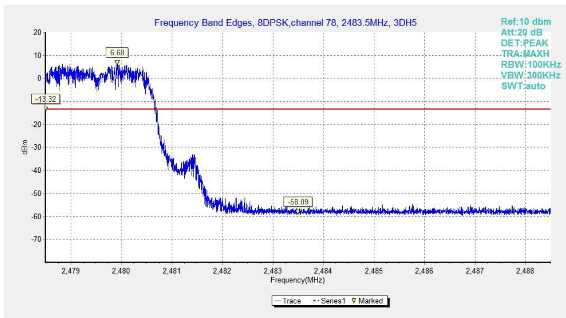
Fig.30. Frequency Band Edges: 8DPSK, Channel 78, Hopping On
