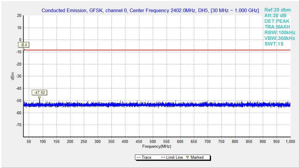
Fig.32. Conducted spurious emission: GFSK, Channel 0, 30MHz - 1GHz
