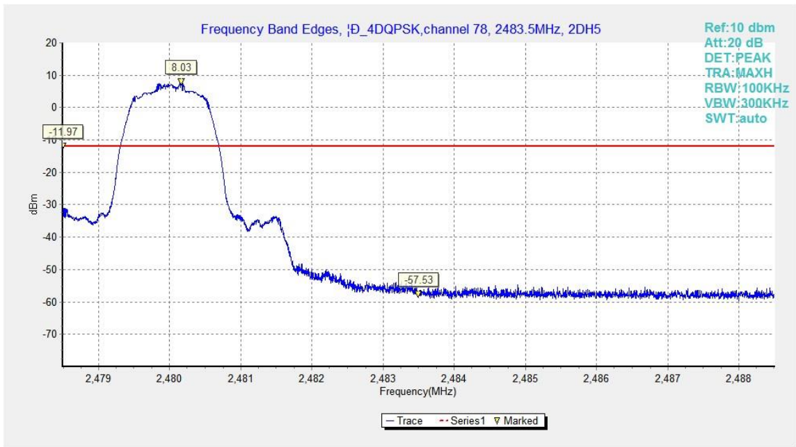
Fig.25. Frequency Band Edges: \pi/4 DQPSK, Channel 78, Hopping Off
