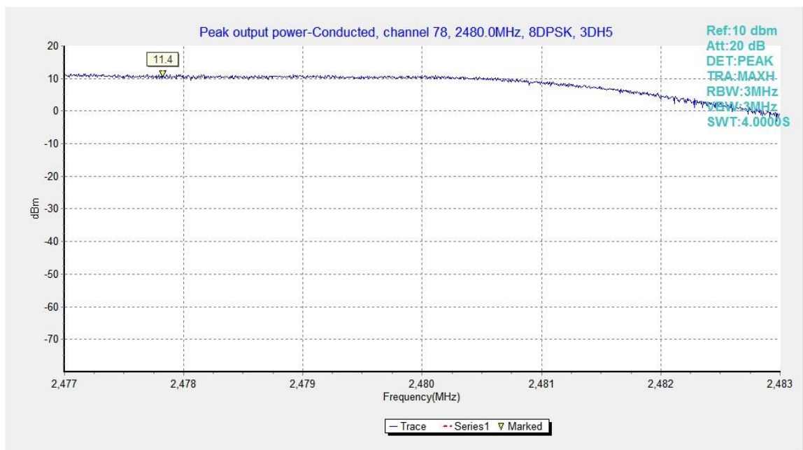
Fig.9. Peak Output Power -Conducted: 8DPSK, Channel 78, ANT0
