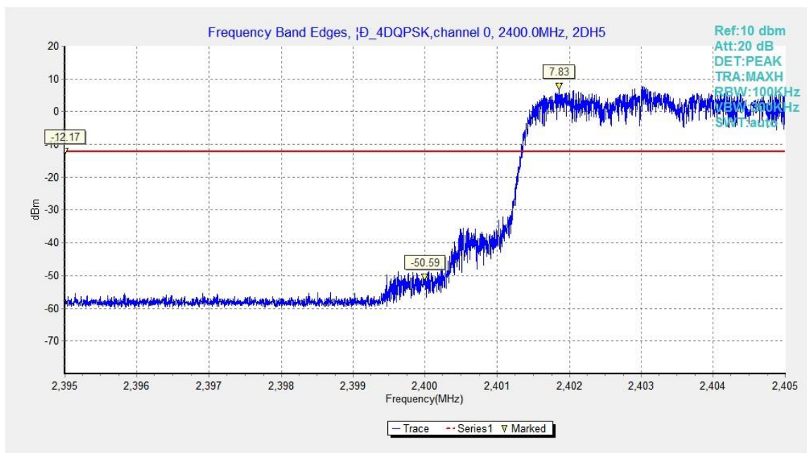
Fig.24. Frequency Band Edges: \pi/4 DQPSK, Channel 0, Hopping On
