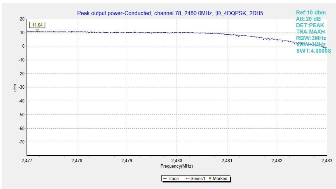
Fig.6. Peak Output Power -Conducted: \pi/4 DQPSK, Channel 78, ANT0
