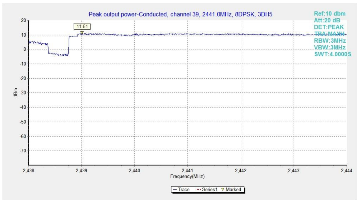
Fig.17. Peak Output Power -Conducted: 8DPSK, Channel 39, ANT1
