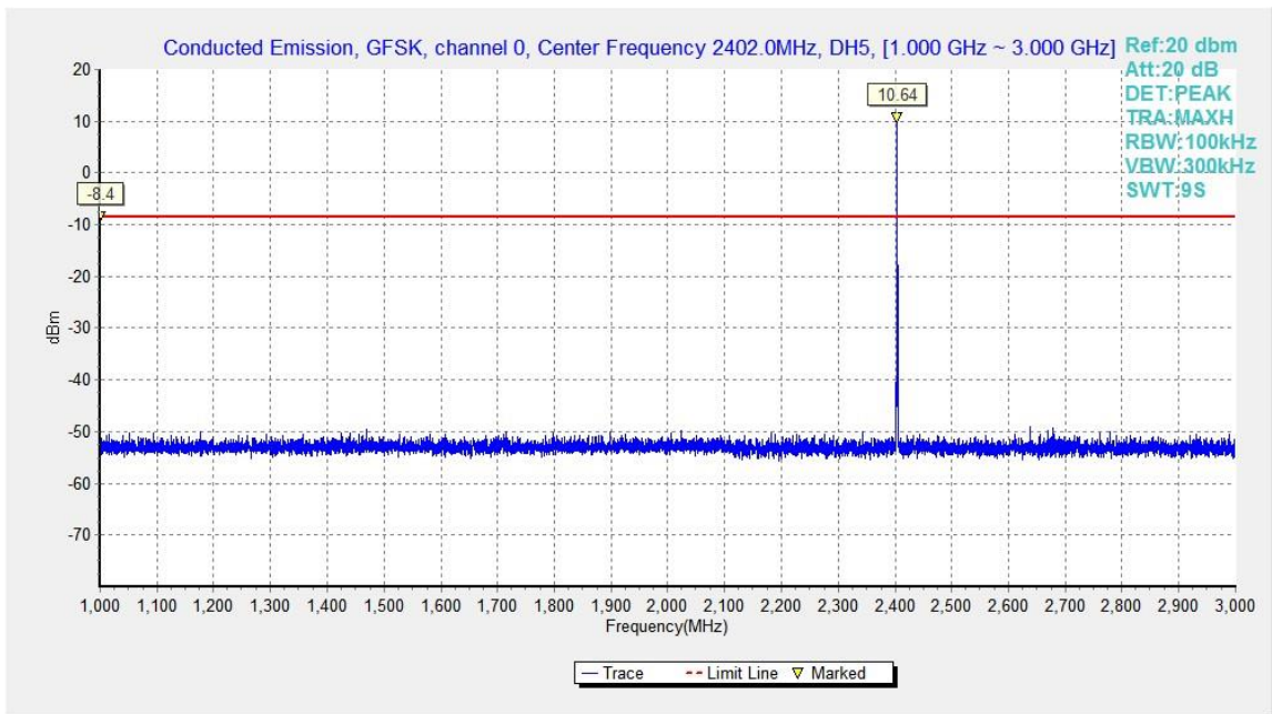
Fig.33. Conducted spurious emission: GFSK, Channel 0, 1GHz - 3GHz
