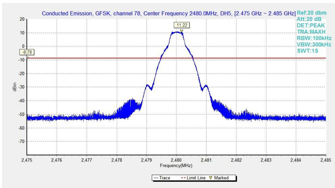
Fig.41. Conducted spurious emission: GFSK, Channel 78, 2480MHz
