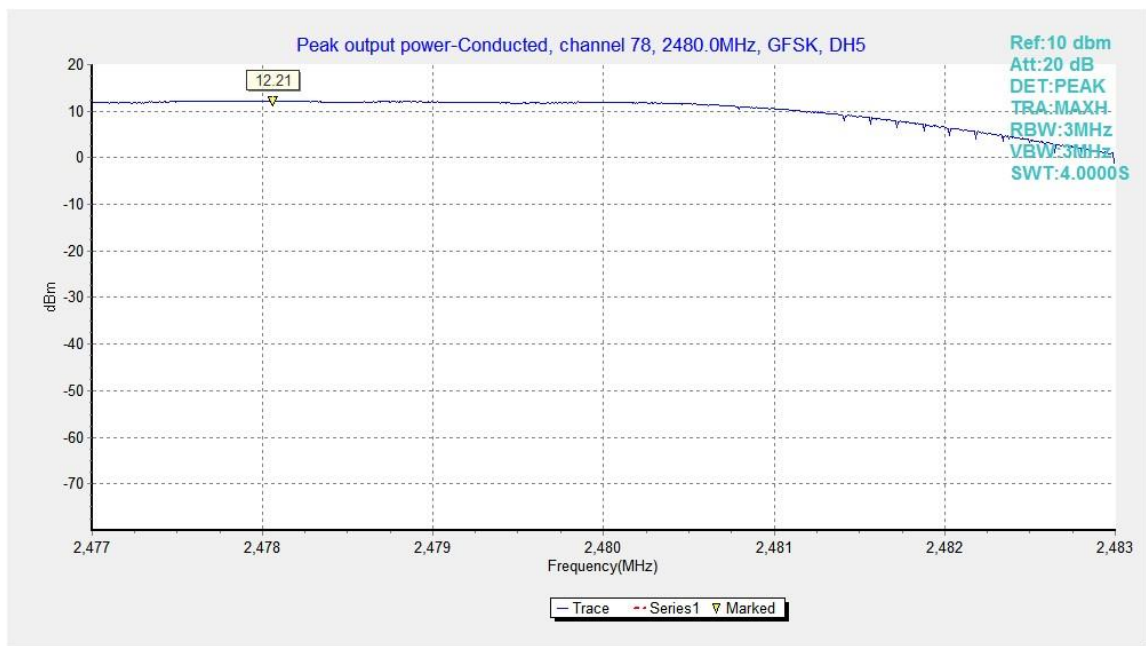
Fig.12. Peak Output Power -Conducted: GFSK, Channel 78, ANT1
