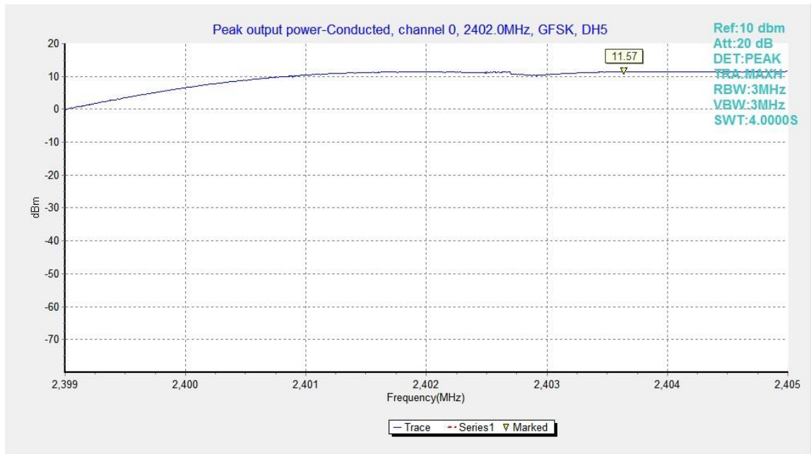
Fig.10. Peak Output Power -Conducted: GFSK, Channel 0, ANT1
