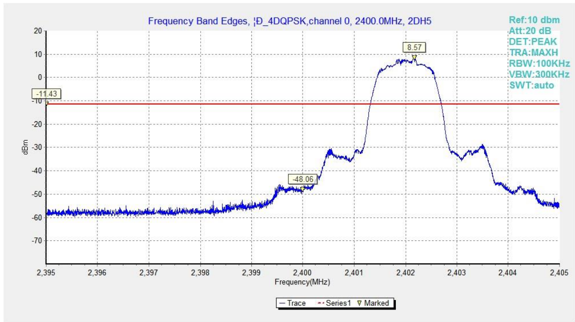
Fig.23. Frequency Band Edges: \pi/4 DQPSK, Channel 0, Hopping Off
