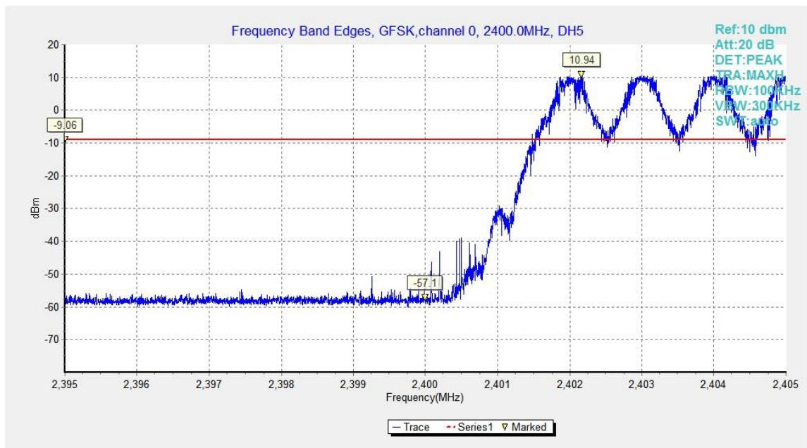
Fig.20. Frequency Band Edges: GFSK, Channel 0, Hopping On
