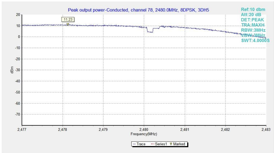
Fig.18. Peak Output Power -Conducted: 8DPSK, Channel 78, ANT1
