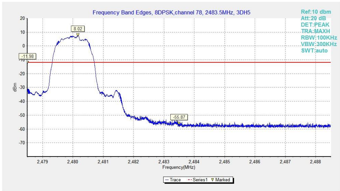
Fig.29. Frequency Band Edges: 8DPSK, Channel 78, Hopping Off
