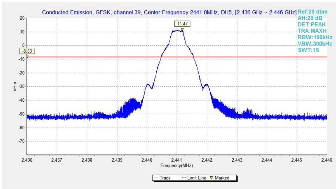
Fig.36. Conducted spurious emission: GFSK, Channel 39, 2441MHz
