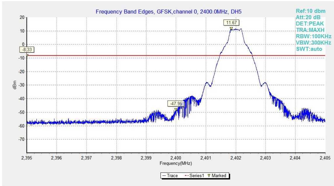
Fig.19. Frequency Band Edges: GFSK, Channel 0, Hopping Off
