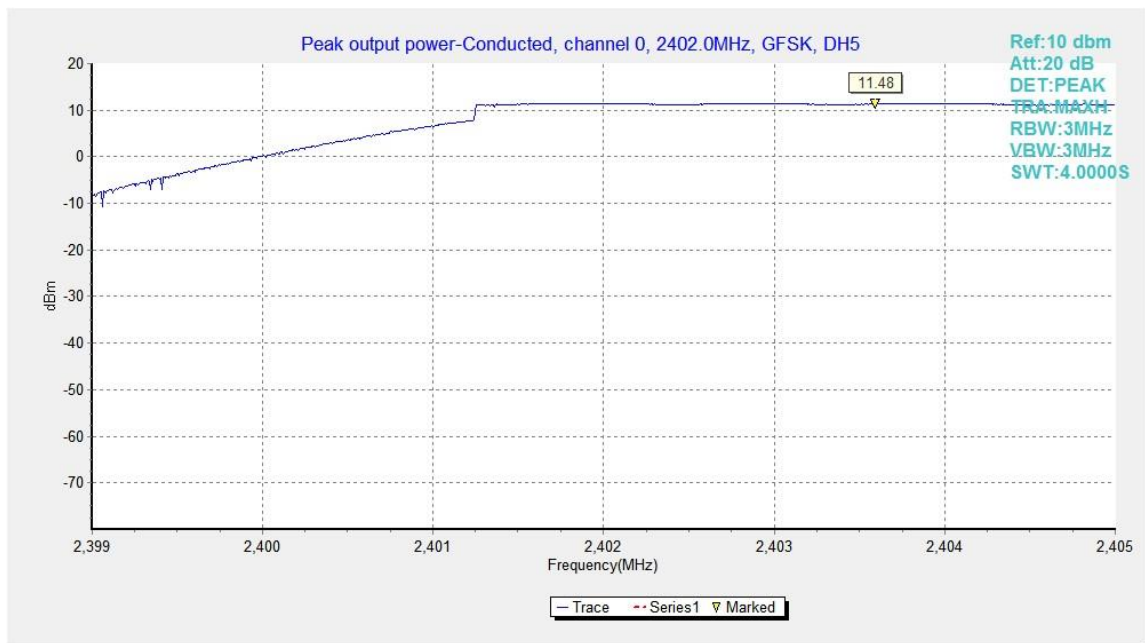
Fig.1. Peak Output Power -Conducted: GFSK, Channel 0, ANT0
