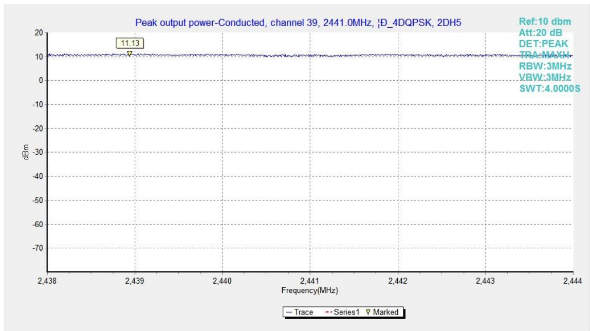
Fig.5. Peak Output Power -Conducted: \pi/4 DQPSK, Channel 39, ANT0
