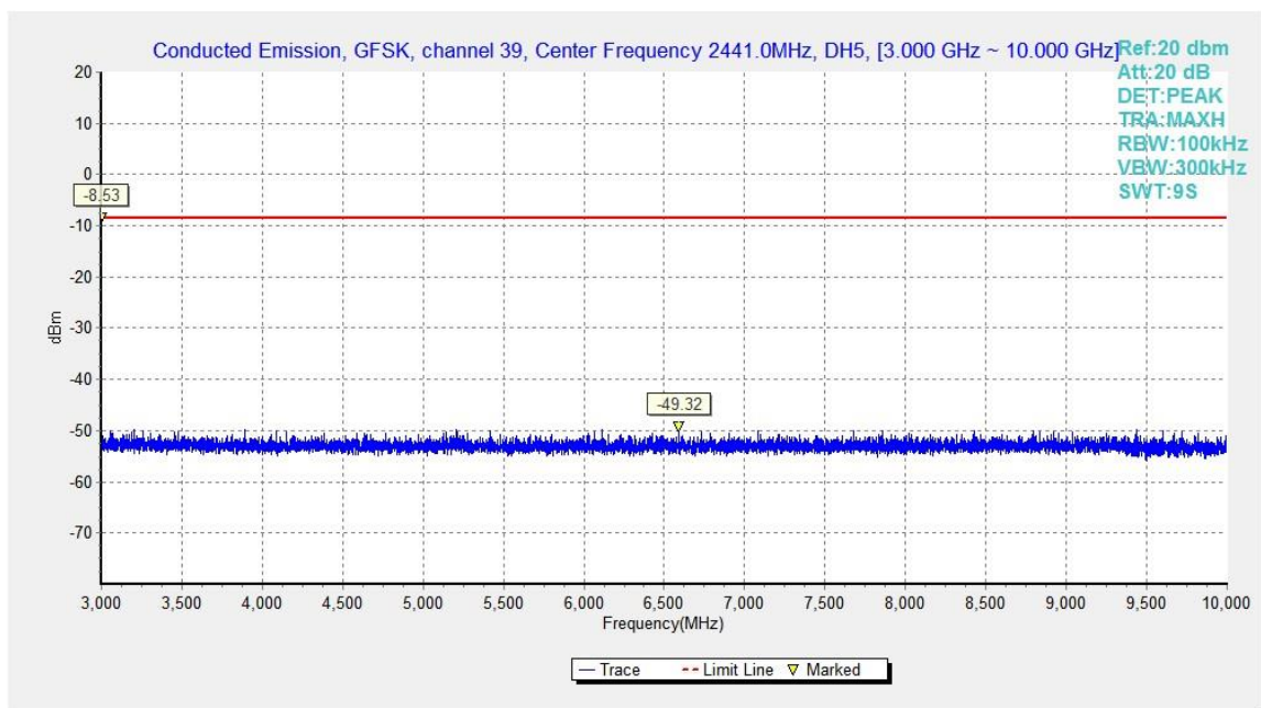
Fig.39. Conducted spurious emission: GFSK, Channel 39, 3GHz – 10GHz
