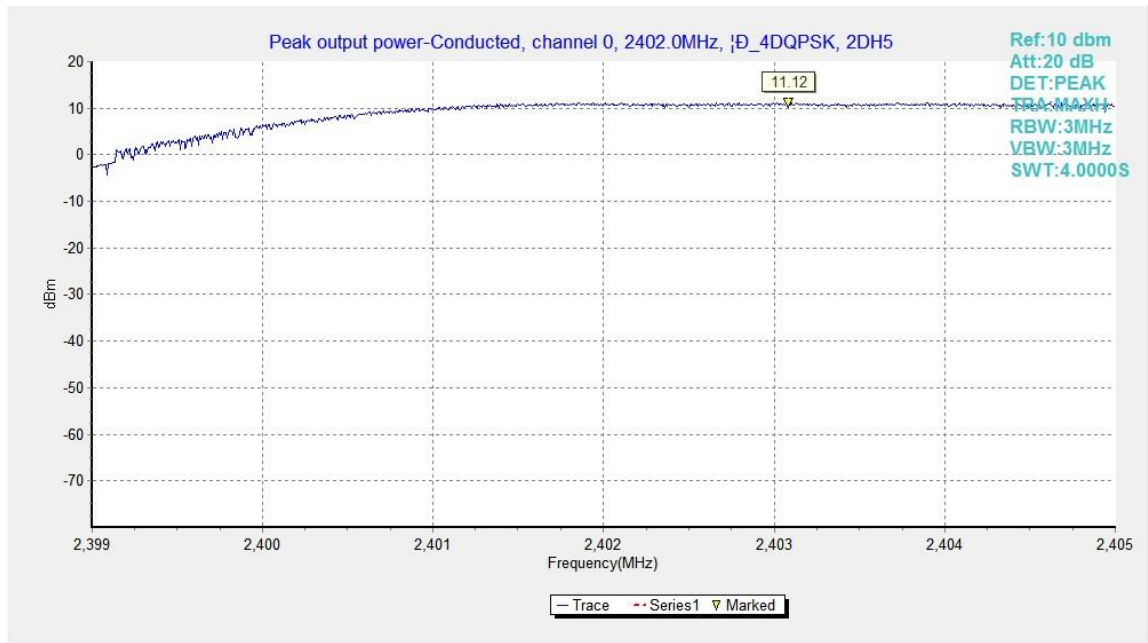
Fig.4. Peak Output Power -Conducted: \pi/4 DQPSK, Channel 0, ANT0
