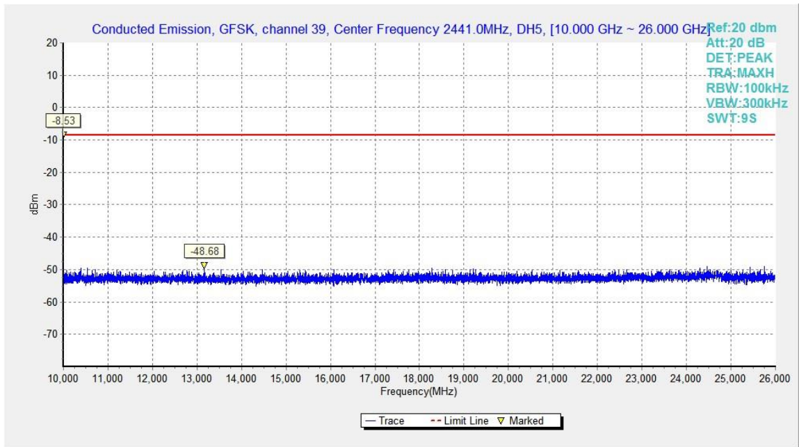
Fig.40. Conducted spurious emission: GFSK, Channel 39, 10GHz – 26GHz
