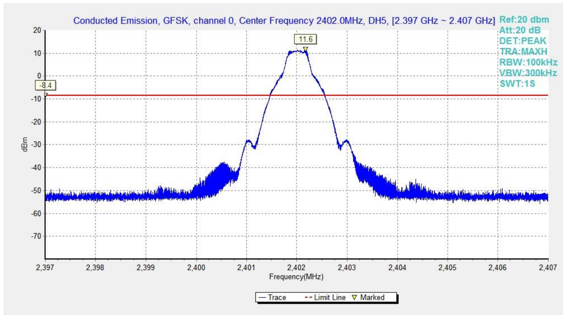
Fig.31. Conducted spurious emission: GFSK, Channel 0, 2402MHz
