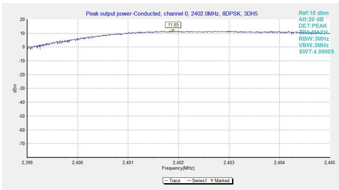
Fig.7. Peak Output Power -Conducted: 8DPSK, Channel 0, ANT0
