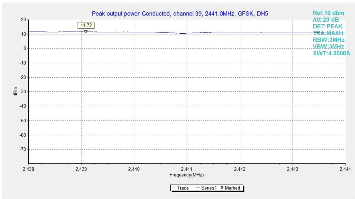
Fig.2. Peak Output Power -Conducted: GFSK, Channel 39, ANT0
