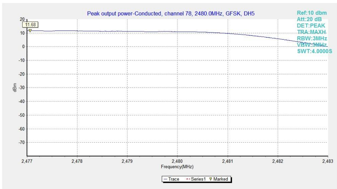
Fig.3. Peak Output Power -Conducted: GFSK, Channel 78, ANT0
