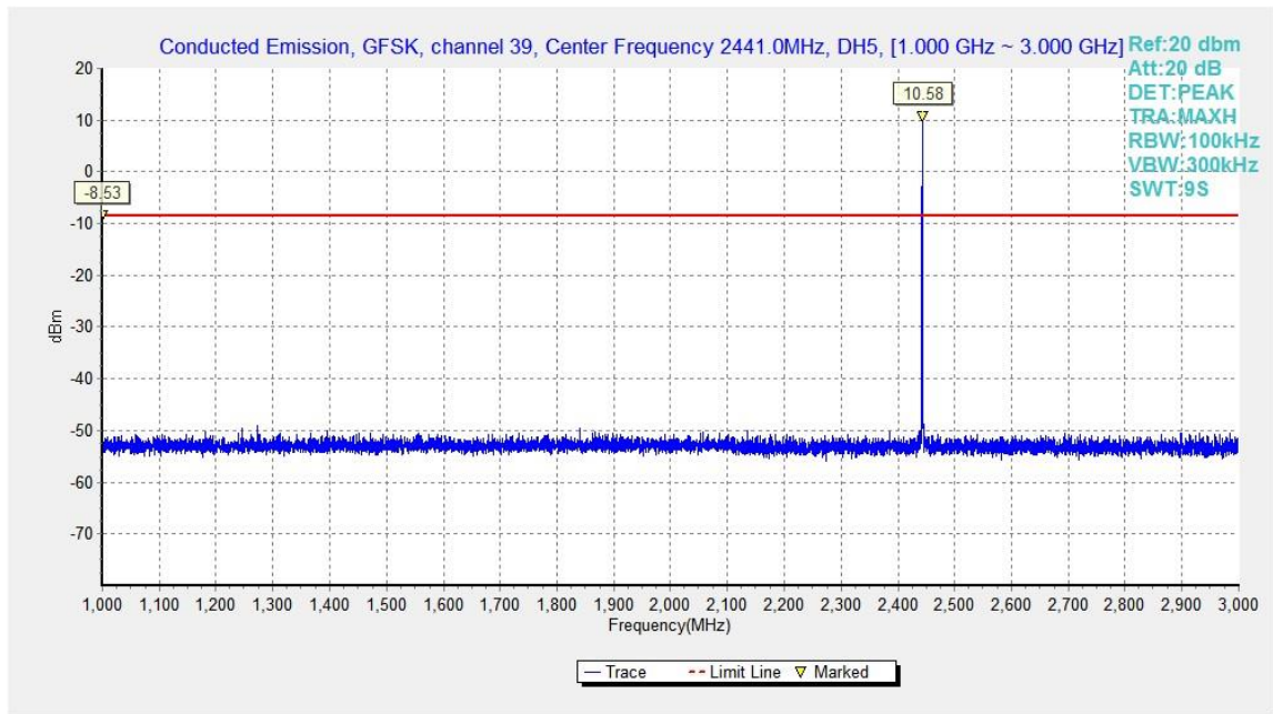
Fig.38. Conducted spurious emission: GFSK, Channel 39, 1GHz – 3GHz
