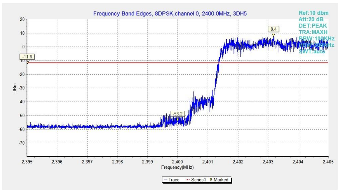
Fig.28. Frequency Band Edges: 8DPSK, Channel 0, Hopping On
