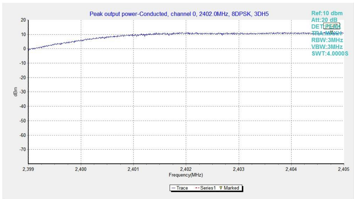
Fig.16. Peak Output Power -Conducted: 8DPSK, Channel 0, ANT1
