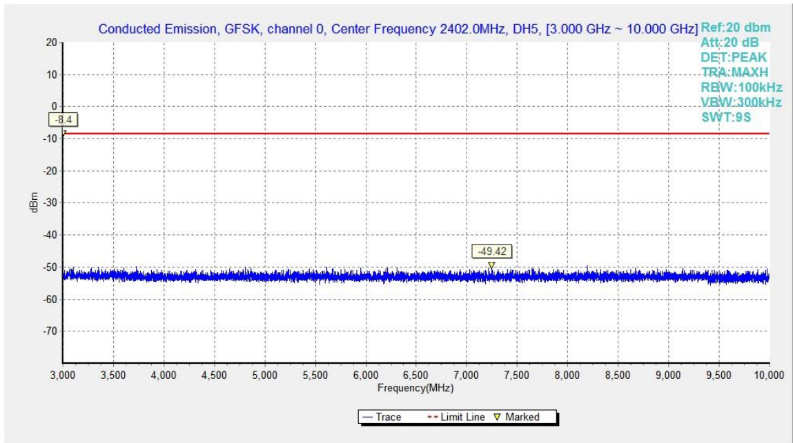
Fig.34. Conducted spurious emission: GFSK, Channel 0, 3GHz - 10GHz
