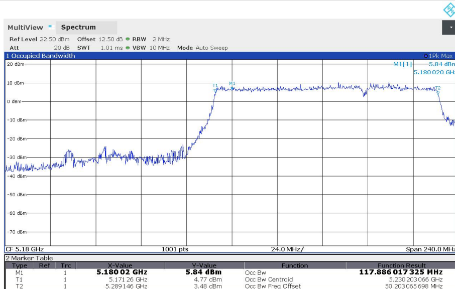
11BE160MIMO_Ant1_5250_Puncturing 20M_7
