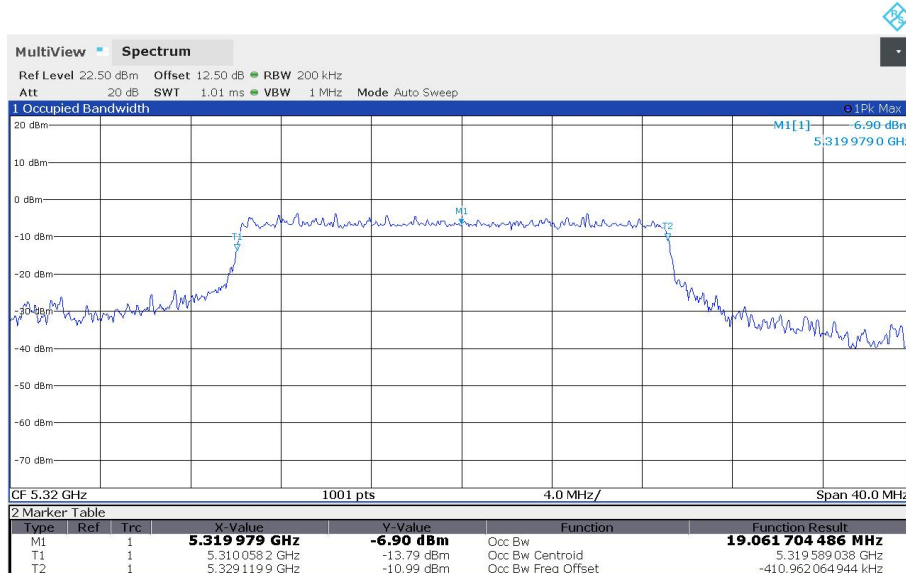
11BE160MIMO_Ant1_5250_Puncturing 20M_7
