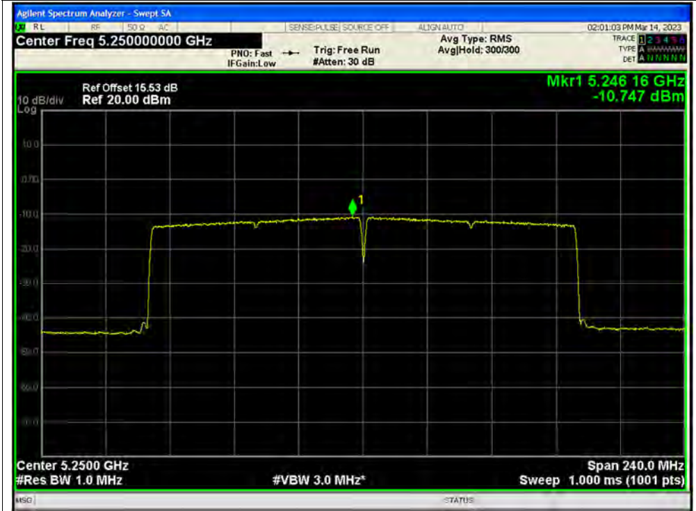
PSD NVNT ax160 5250MHz Ant3
