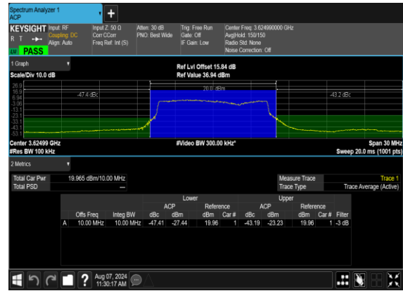
N48(10M)_DFT-s-OFDM_QPSK_Outer_Full_Mid_CH
