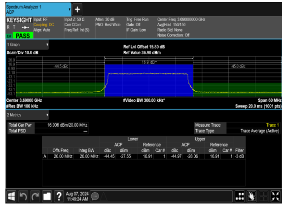
N48(20M)_DFT-s-OFDM_QPSK_Outer_Full_High_CH
