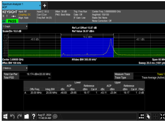
N48(20M)_DFT-s-OFDM_PI_2-BPSK_Edge_1RB_Right_High_CH
