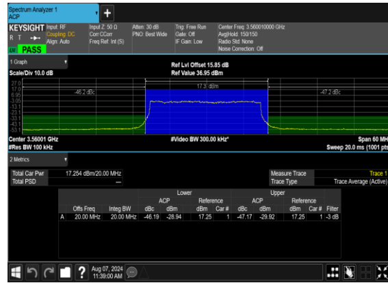
N48(20M)_DFT-s-OFDM_QPSK_Outer_Full_Low_CH
