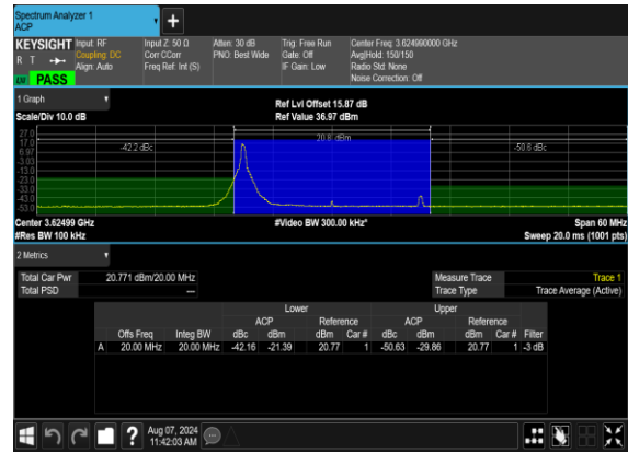
N48(20M)_DFT-s-OFDM_PI_2-BPSK_Edge_1RB_Left_Mid_CH
