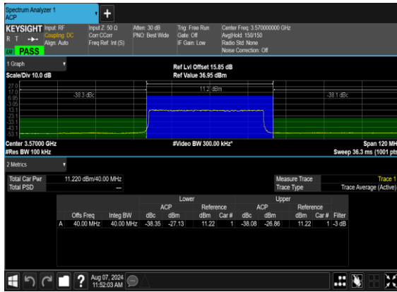
N48(40M)_DFT-s-OFDM_PI_2-BPSK_Outer_Full_Low_CH
