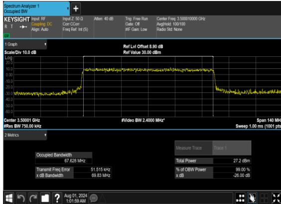
N77(70M)_CP-OFDM_64 QAM_Outer_Full_Mid_CH
