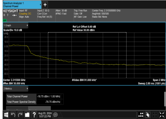
N30(5M)_DFT-s-OFDM_QPSK_Outer_Full_High_CH_CHP_PASS
