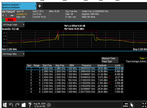
N30(10M)_DFT-s-OFDM_BPSK_Outer_Full_Low_CH
