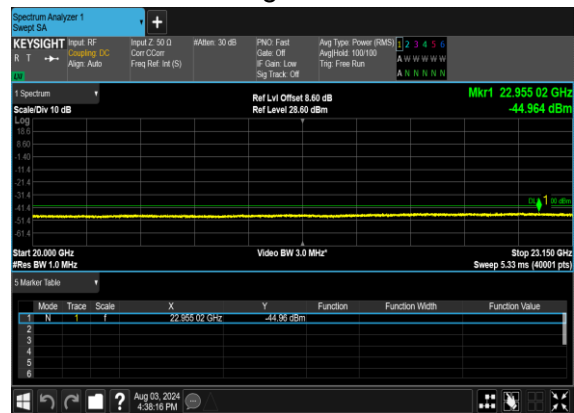
N30(5M)_DFT-s-OFDM_BPSK_Edge_1RB_Left_Mid_CH
