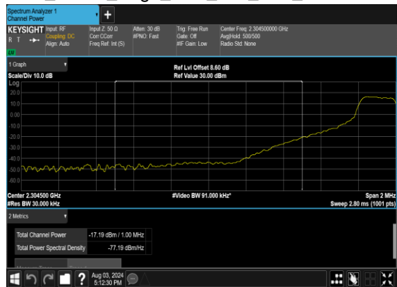
N30(10M)_DFT-s-OFDM_QPSK_Edge_1RB_Left_Low_CH_CHP_PASS
