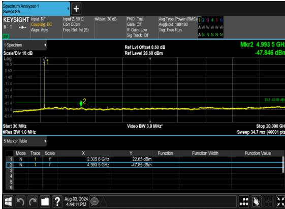
N30(10M)_DFT-s-OFDM_BPSK_Edge_1RB_Left_Low_CH
