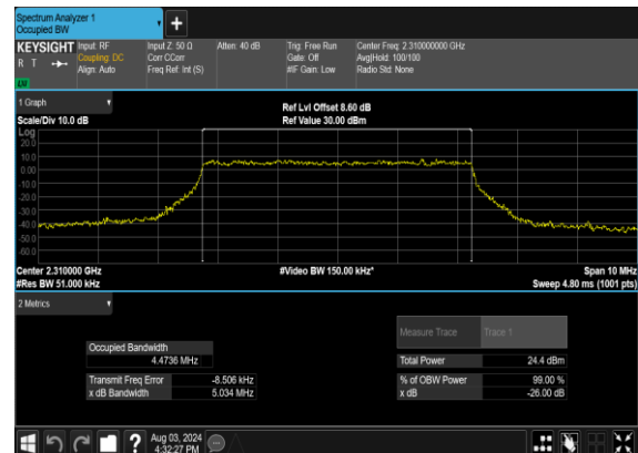
N30(5M)_CP-OFDM_256 QAM_Outer_Full_Mid_CH
