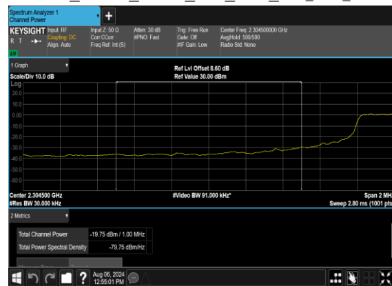
N30(10M)_DFT-s-OFDM_BPSK_Outer_Full_Low_CH_CHP_PASS
