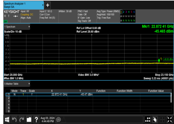
N30(10M)_DFT-s-OFDM_BPSK_Edge_1RB_Left_Low_CH
