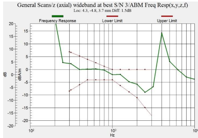
Figure C.7 Frequency Response of LTE B7 - OTT VoIP
