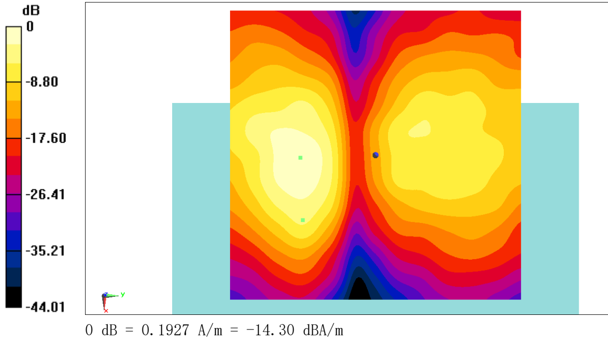
Fig B.19 T-Coil WiFi-5G
