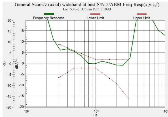
Figure C.8 Frequency Response of LTE B41 PC2 - OTT VoIP
