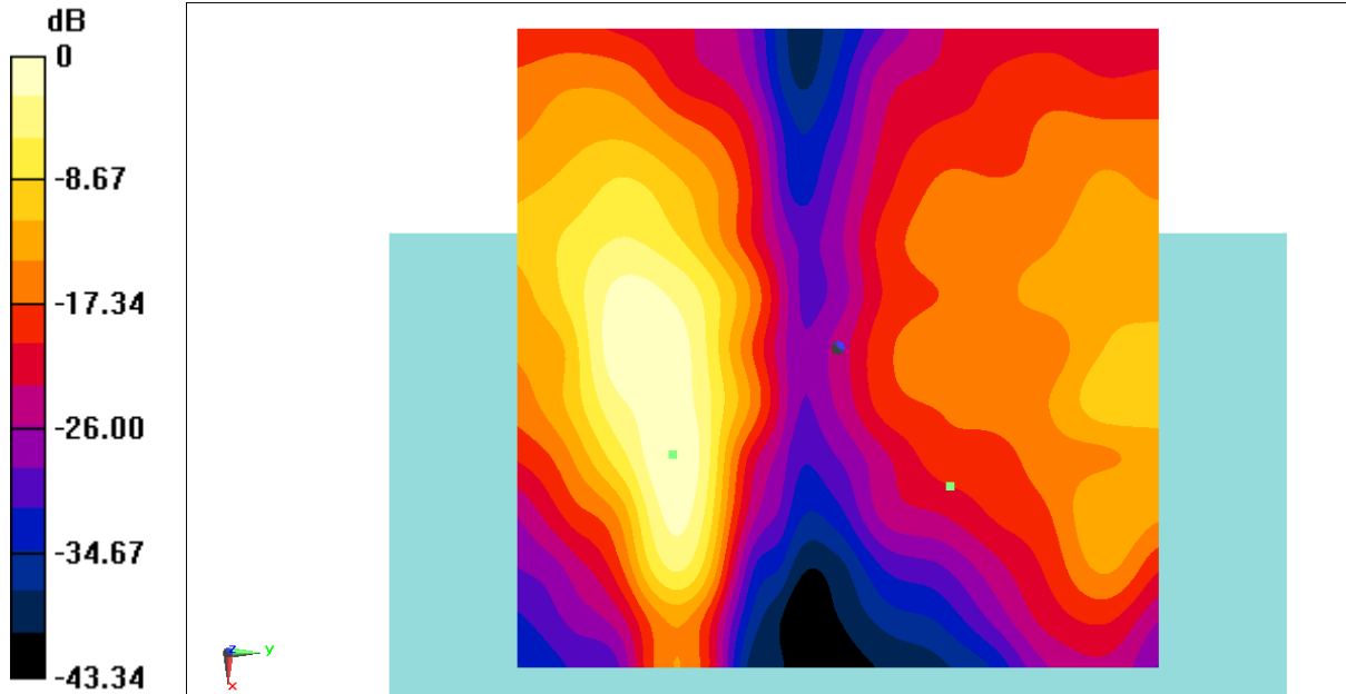
Fig B.17 T-Coil WiFi-2.4G
