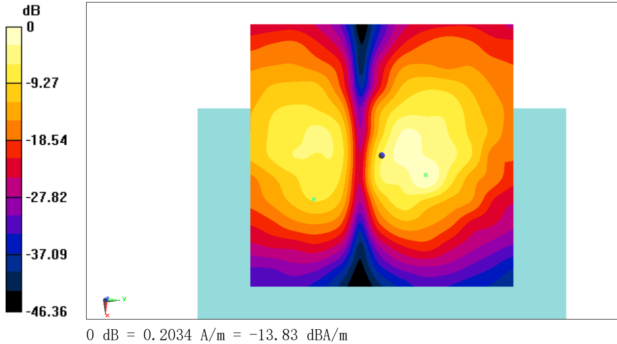
Fig B.13 T-Coil LTE B7
