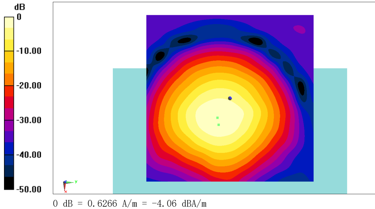
Fig B.10 T-Coil WiFi-5G
