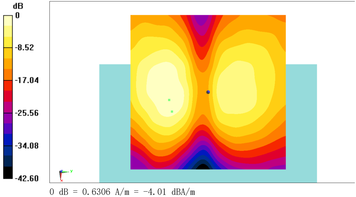
Fig B.15 T-Coil LTE B41
