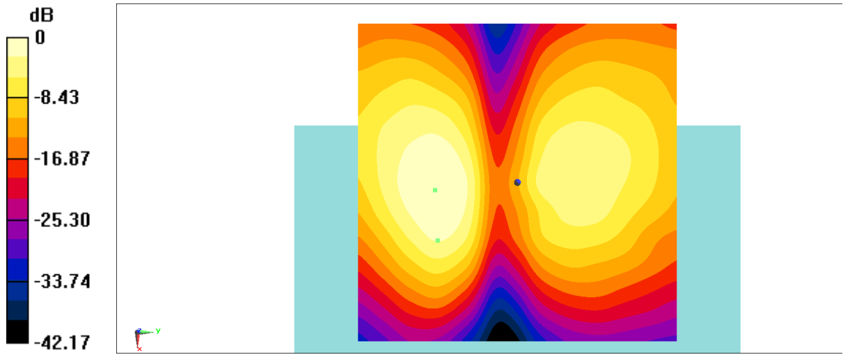
Fig B.3 T-Coil LTE B2
