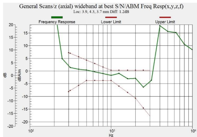
Figure C.6 Frequency Response of EDGE850 - OTT VoIP
