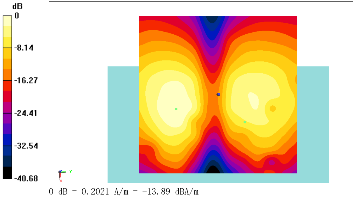
Fig B.9 T-Coil WiFi-5G
