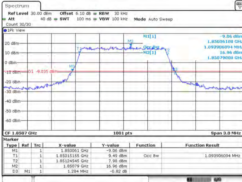
Band25-1.4MHz-QPSK-26047-6RB#0-1.094
