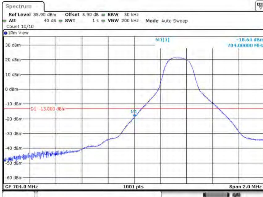
Band17-5MHz-QPSK-23755-1RB#0
