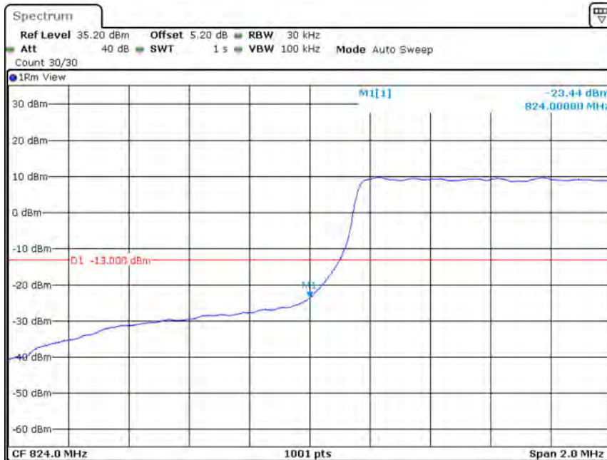
Band26-1.4MHz-QPSK-26797-6RB#0
