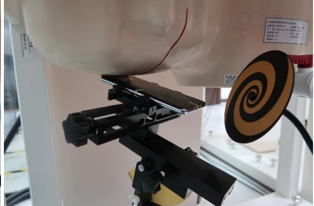
Head, Right Tilted, Separation distance 0mm
