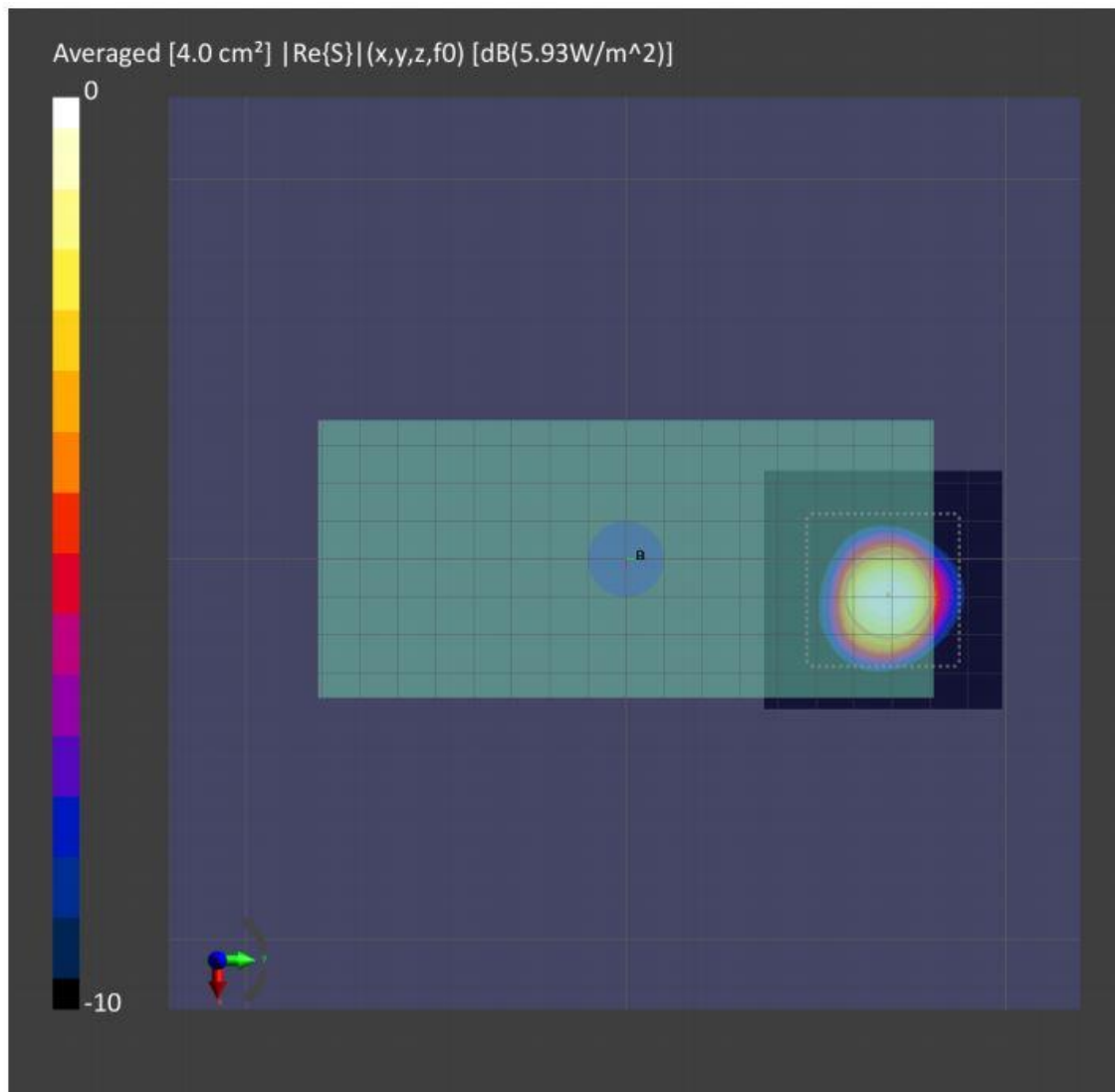
Figure 8-4: 4cm2-averaged power density distribution measured at input.power.limit of 3.61dBm on the back surface for n261 beam 23
