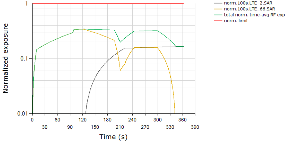
Total Normalized Time-averaged RF Exposure Tech: LTE, Band 2 / Tech: LTE, Band 66
