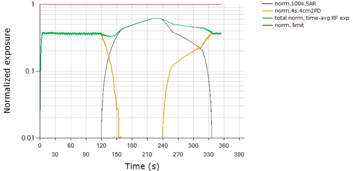
Total Normalized Time-averaged RF Exposure Tech: LTE, Band 2 / Tech: NR5G MMW, Band n258
