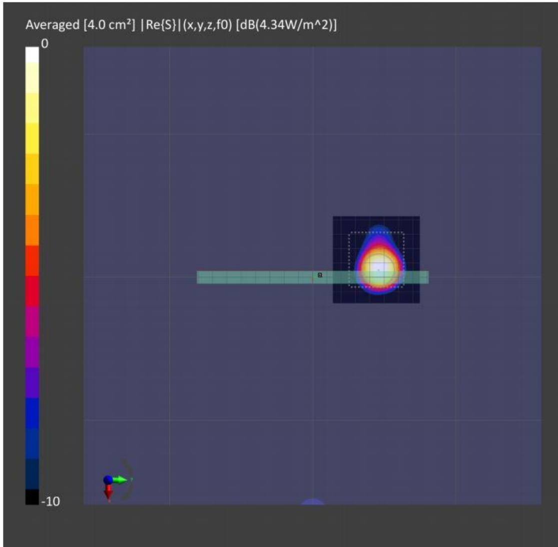
Figure 8-2: 4cm2-averaged power density distribution measured at input.power.limit of 3.88 dBm on the Right Side surface for n258 beam 39
