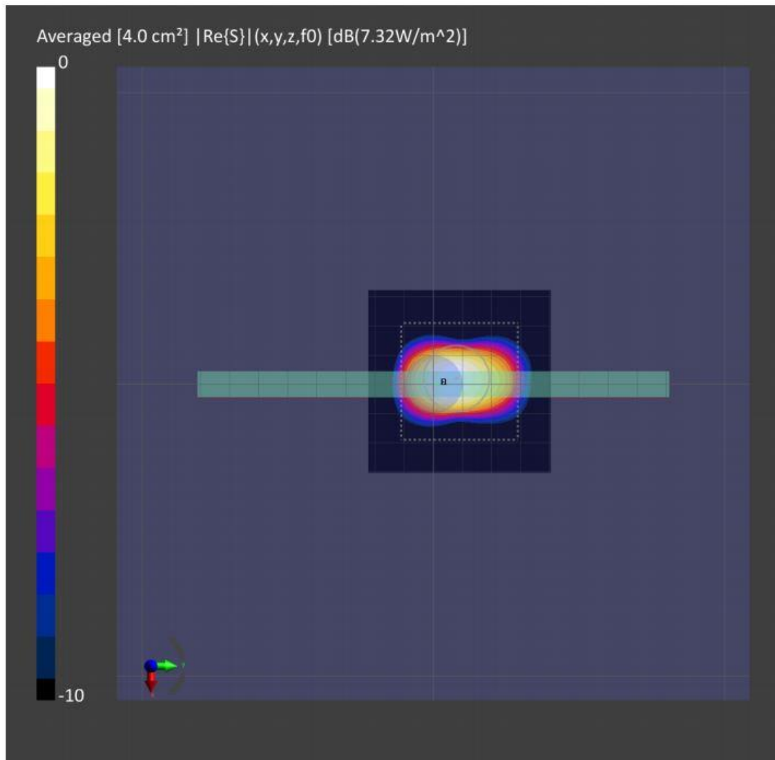
Figure 8-3: 4cm2-averaged power density distribution measured at input.power.limit of 4.68 dBm on the Back for n260 beam 35
