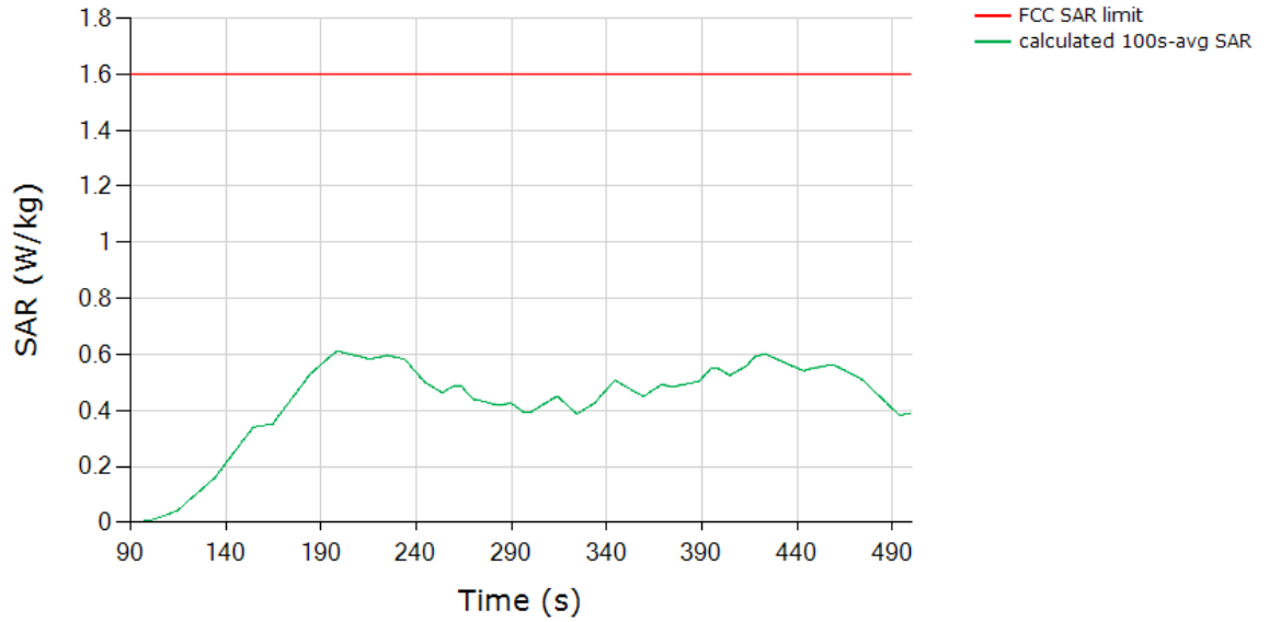
SAR (Test Sequence 2) Tech: GSM, Band GSM 1900
