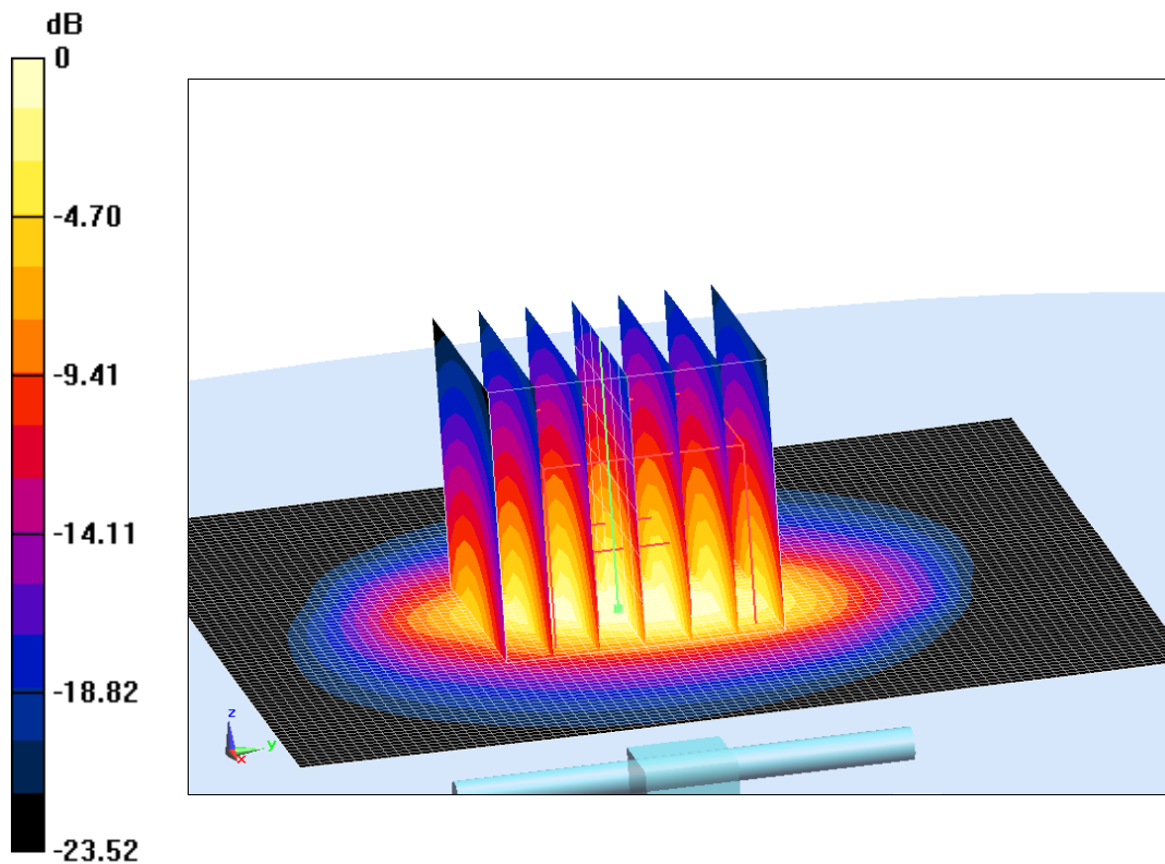
Fig.J.4 validation 2600 MHz 250mW
