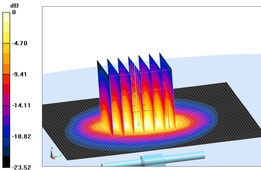
Fig.J.3 validation 2600 MHz 250Mw
