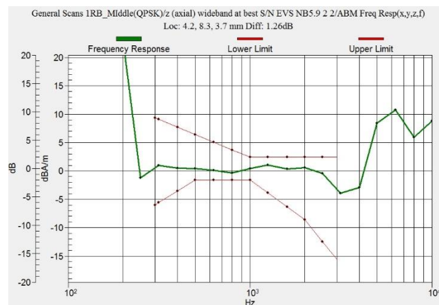
Figure C.18 Frequency Response of LTE B41 Power Class 3
