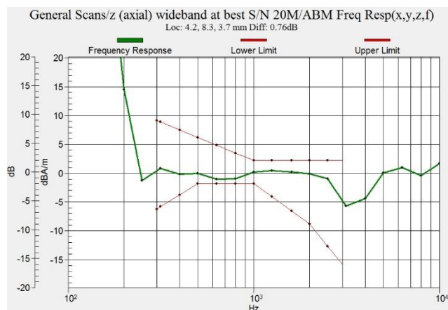
Figure C.15 Frequency Response of LTE B66
