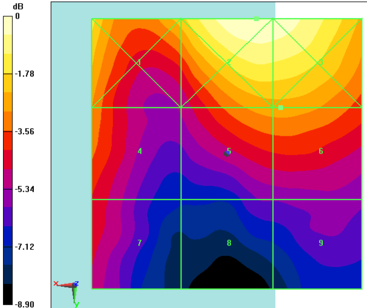
Fig B.37 HAC RF E-Field LTE Band41 Power Class 2 64QAM CH40620
