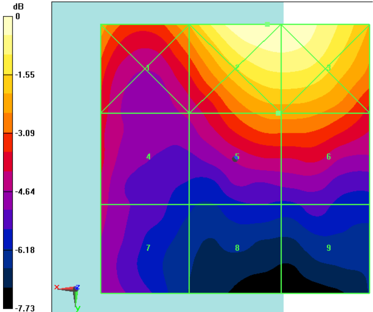
Fig B.43 HAC RF E-Field LTE Band41 Power Class 3 QPSK CH40185
