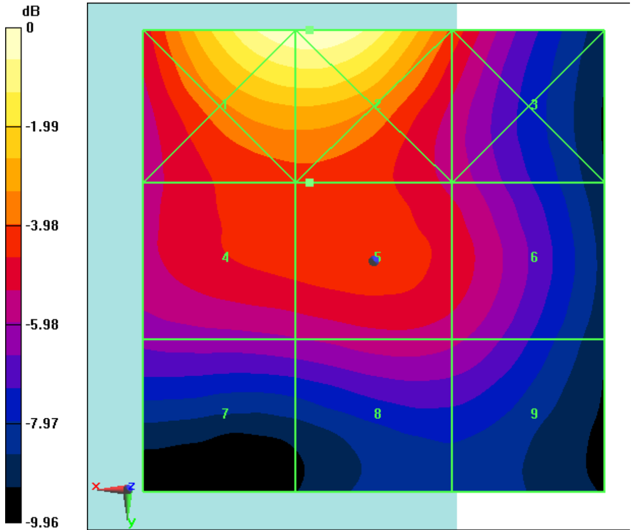
Fig B.16 HAC RF E-Field LTE Band48 QPSK CH56640
