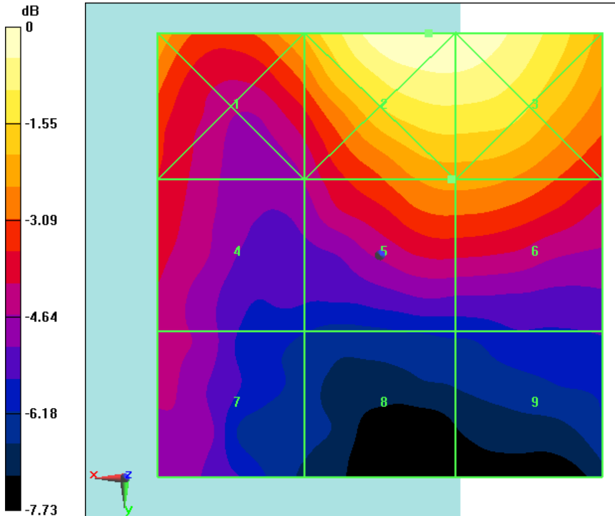
Fig B.33 HAC RF E-Field LTE Band41 Power Class 2 16QAM CH40185
