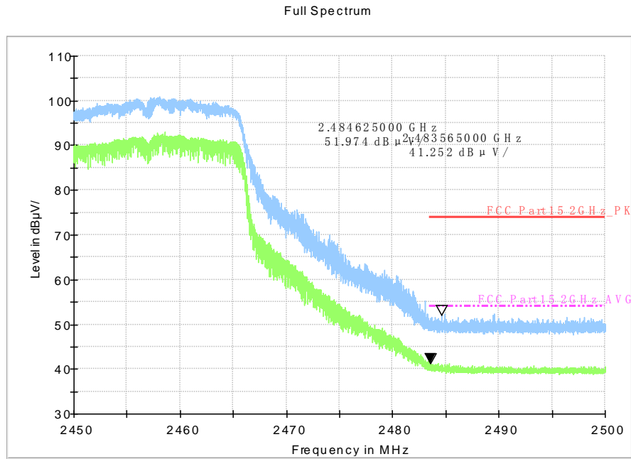
Fig.A.6.2.10 Transmitter Spurious Emission - Radiated (Power): 802.11n-HT20, ch10, 2.45 GHz - 2.50GHz
