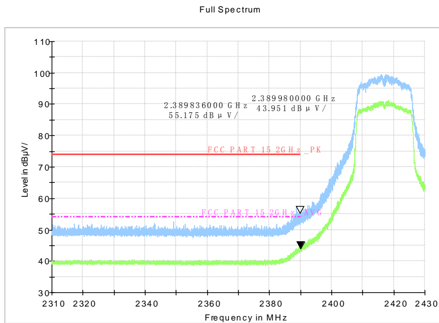
Fig.A.6.2.9 Transmitter Spurious Emission - Radiated (Power): 802.11n-HT20, ch2, 2.31 GHz - 2.43GHz
