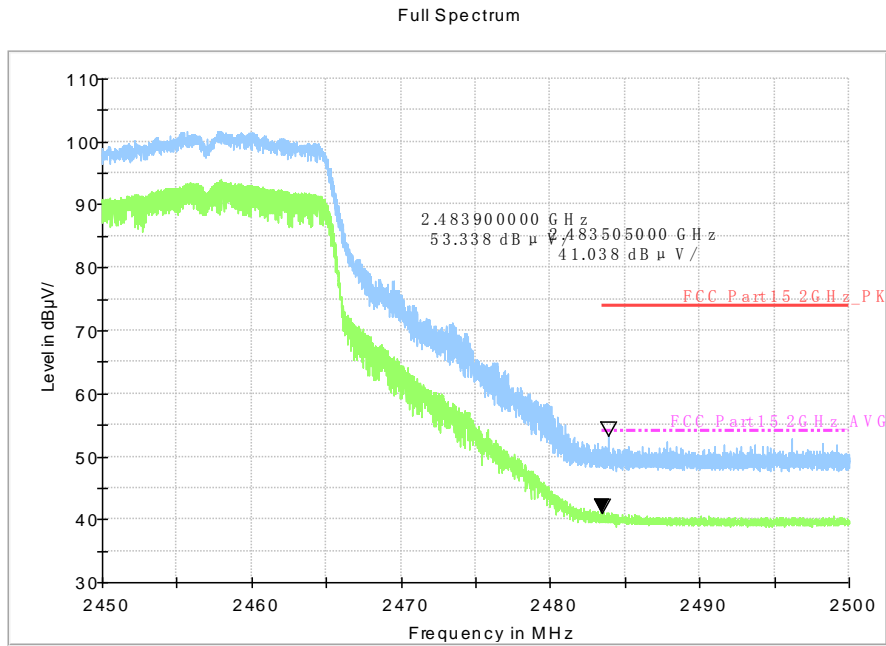
Fig.A.6.2.6 Transmitter Spurious Emission - Radiated (Power): 802.11g, ch10, 2.45 GHz - 2.50GHz
