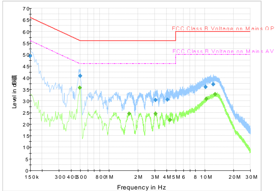
Fig.A.7.3 AC Powerline Conducted Emission-802.11b Ant0+Ant1
