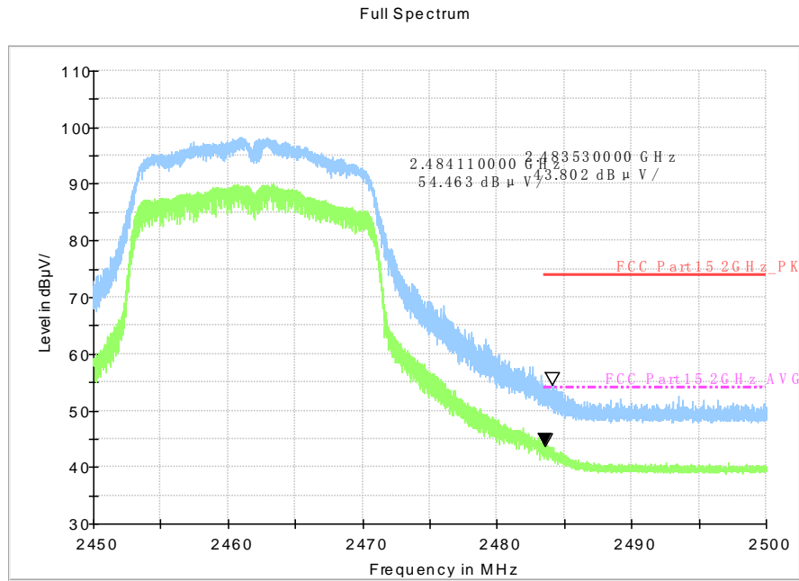
Fig.A.6.2.8 Transmitter Spurious Emission - Radiated (Power): 802.11n-HT20, ch11, 2.45 GHz - 2.50GHz
