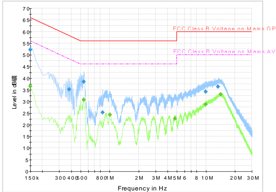
Fig.A.7.1 AC Powerline Conducted Emission-802.11b Ant0+Ant1
