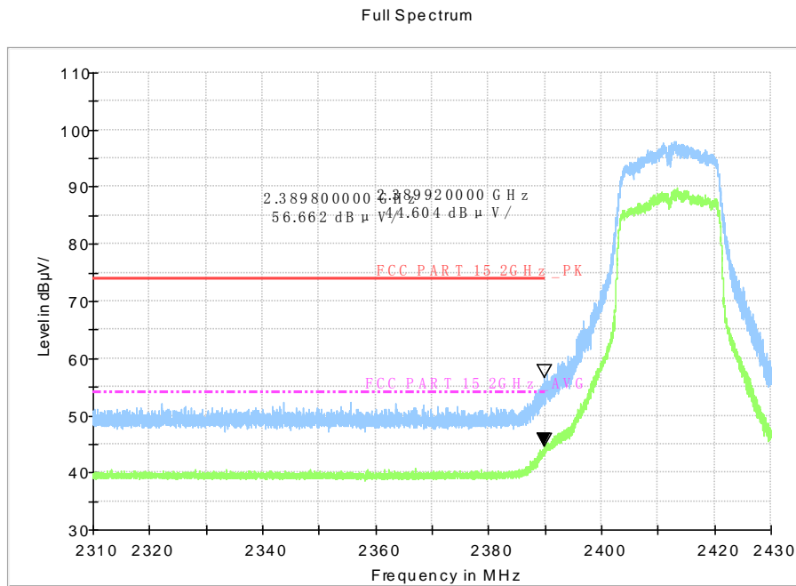
Fig.A.6.2.7 Transmitter Spurious Emission - Radiated (Power): 802.11n-HT20, ch1, 2.31 GHz - 2.43GHz
