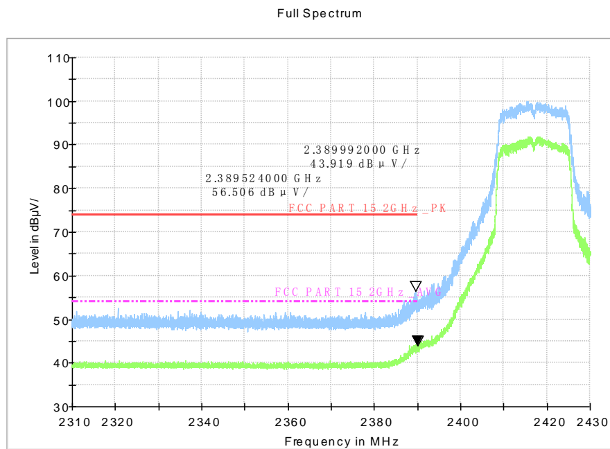
Fig.A.6.2.5 Transmitter Spurious Emission - Radiated (Power): 802.11g, ch2, 2.31 GHz - 2.43GHz
