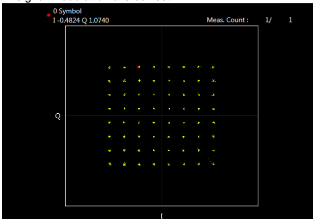
64QAM
