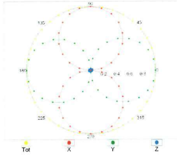
f=1800 MHz,R22,0°
