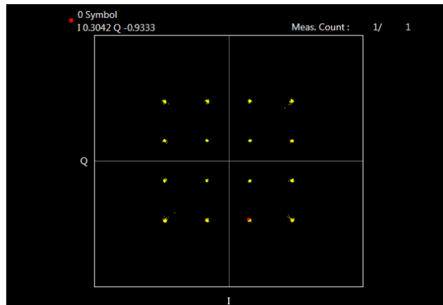
16QAM
