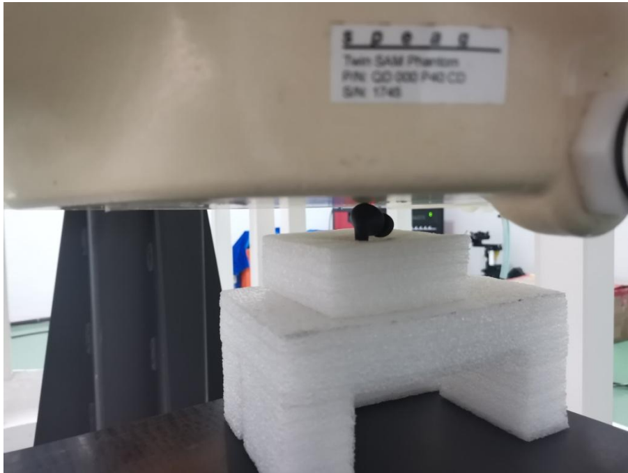
Right earphone-Top Face
