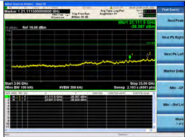
GFSK MIDDLE CHANNEL, SPURIOUS 3 GHz ~ 25 GHz
