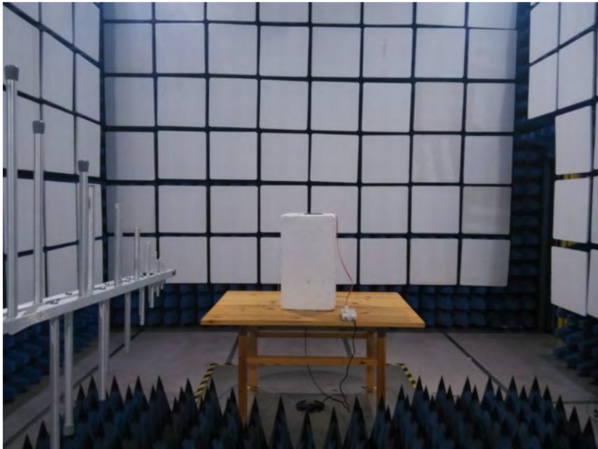
30 MHz-1 GHz
