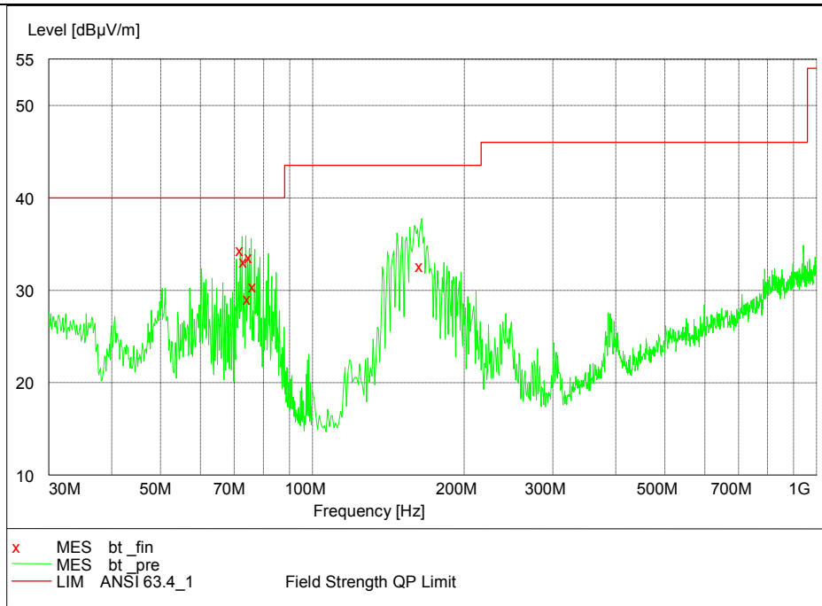
Frequency Range: 30MHz-1000 MHz Detector: QP mode Modulation type: \pi/4 DQPSK
