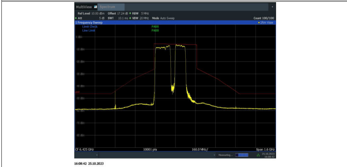
11BE320MIMO_Ant15_6425_2*996+484_OFDMA_5
