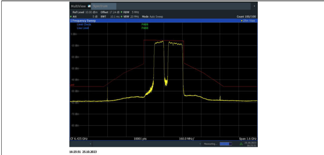
11BE320MIMO_Ant15_6425_2*996+484_OFDMA_10
