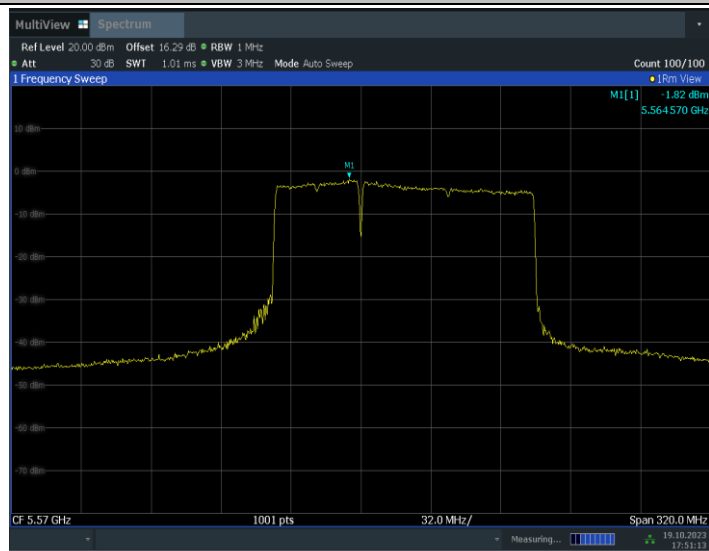
11BE160MIMO_Ant15_5570_996+484_OFDMA_1
