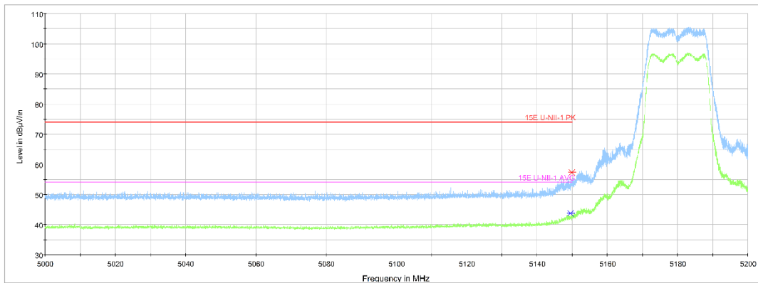
Fig. 1 Band Edges (802.11a MIMO, Ch36, 5180MHz)
