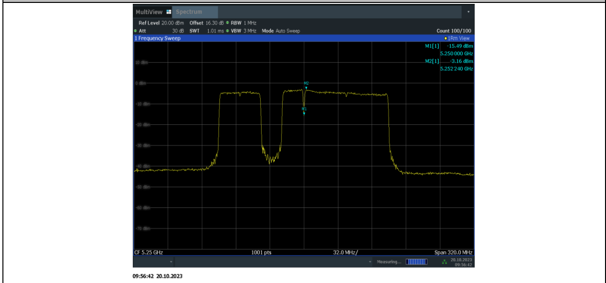
11BE160MIMO_Ant15_5250_UNII-2A_996+484+242_OFDMA_4
