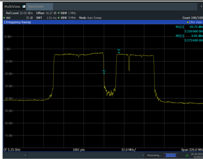
11BE160MIMO_Ant15_5250_UNII-2A_996+484+242_OFDMA_5
