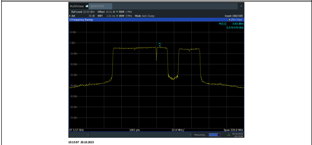
11BE160MIMO_Ant9_5570_996+484+242_OFDMA_7
