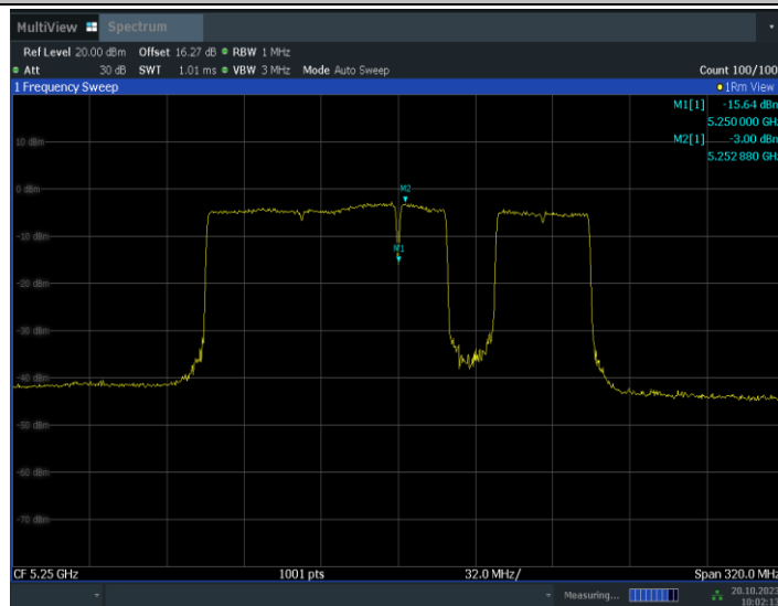
11BE160MIMO_Ant15_5250_UNII-2A_996+484+242_OFDMA_6
