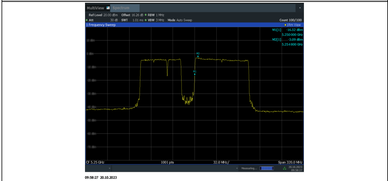
11BE160MIMO_Ant15_5250_UNII-2A_996+484+242_OFDMA_4
