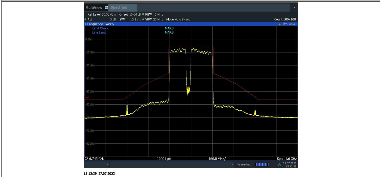
11BE320MIMO_Ant1_6745_996+996+996+484_5
