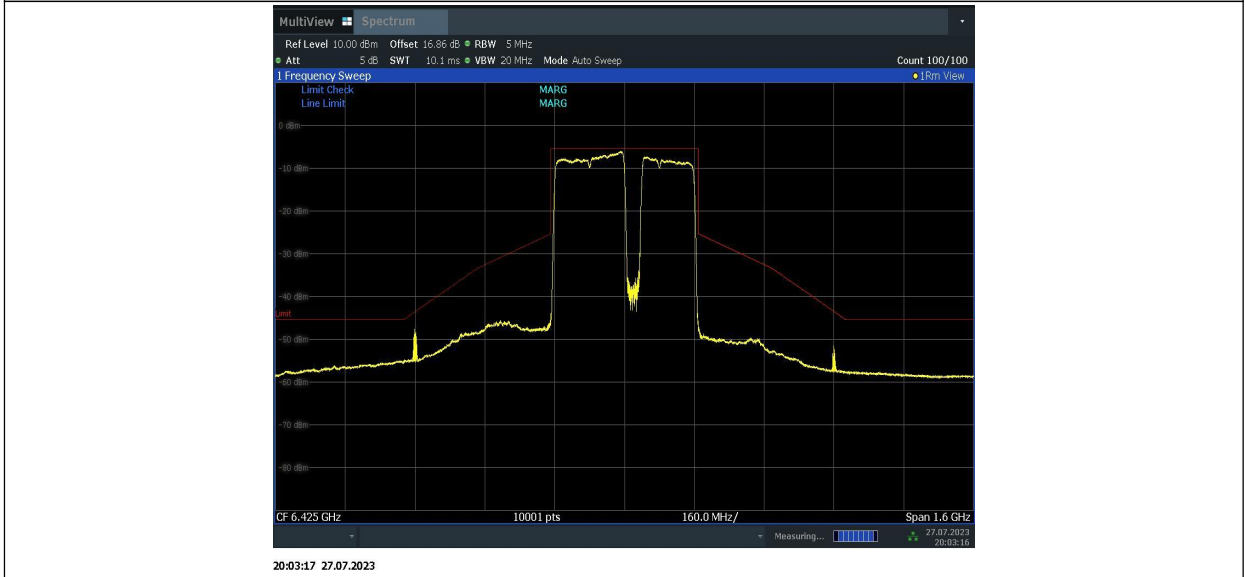
11BE320MIMO_Ant1_6425_996+996+996+484_6
