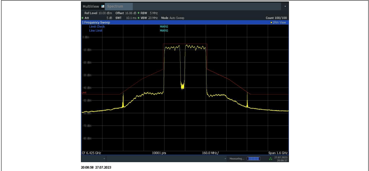
11BE320MIMO_Ant1_6425_996+996+996+484_5
