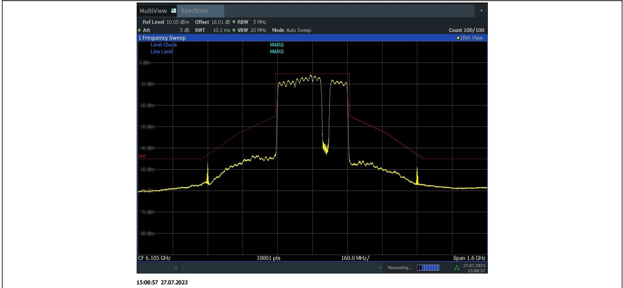
11BE320MIMO_Ant1_6105_996+996+996+484_7
