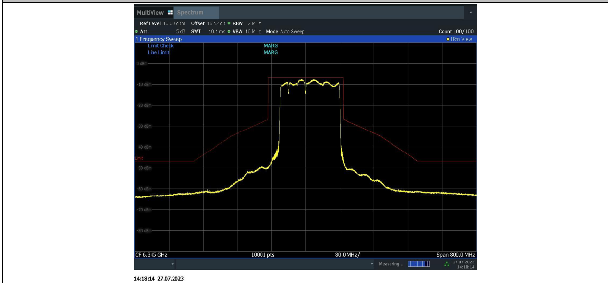
11BE160MIMO_Ant1_6345_996+484+242_1
