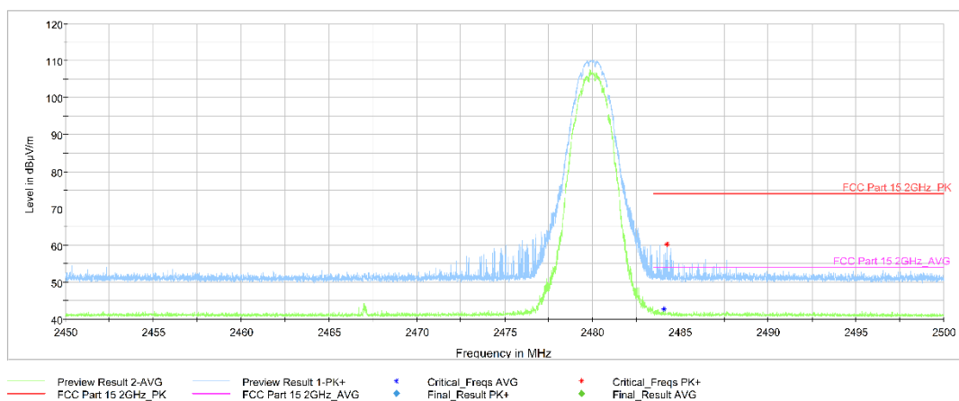
Fig.16. Frequency Band Edges: \pi/4 DQPSK, Channel 78, Hopping Off, 2.45 GHz - 2.50GHz, SISO chain 0, unfolded
