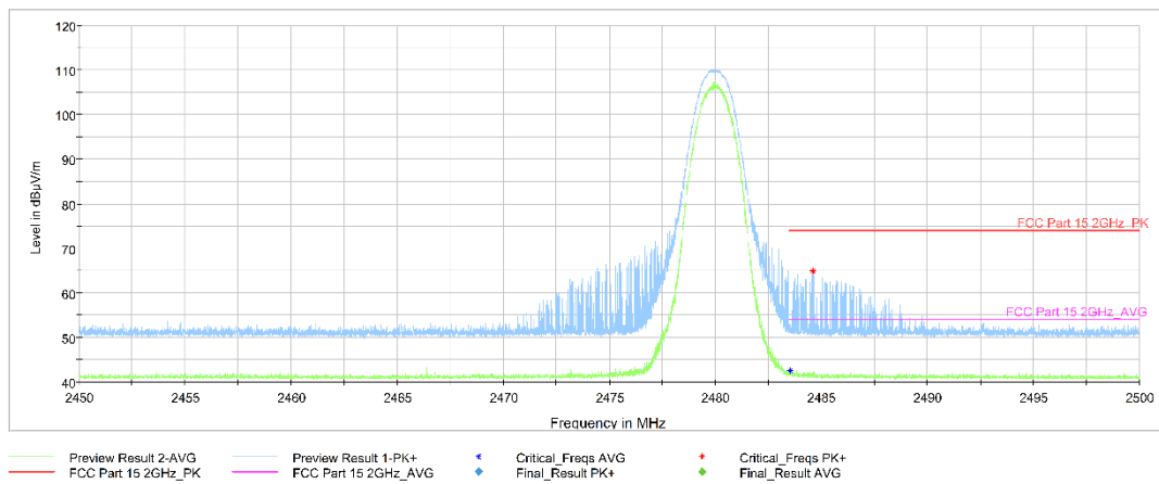
Fig.18. Frequency Band Edges: 8DPSK, Channel 78, 2.45 GHz - 2.50GHz, SISO chain 0, unfolded
