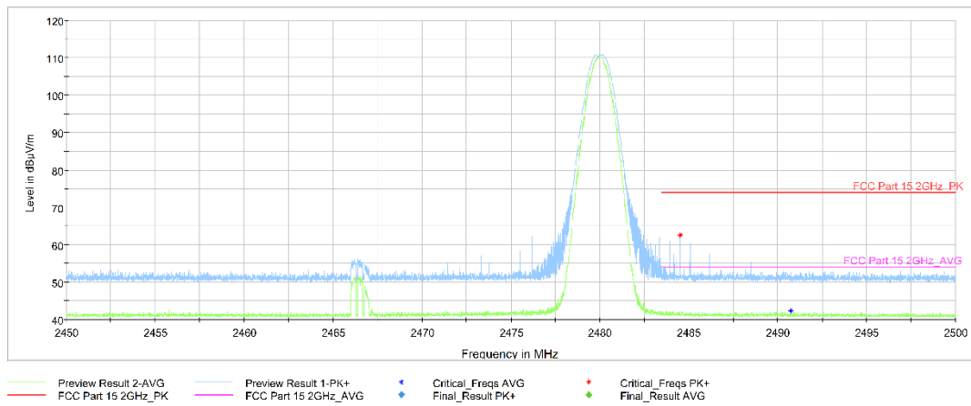
Fig.14. Frequency Band Edges: GFSK, Channel 78, Hopping Off, ch11, 2.45 GHz - 2.50GHz, SISO chain 0, unfolded
