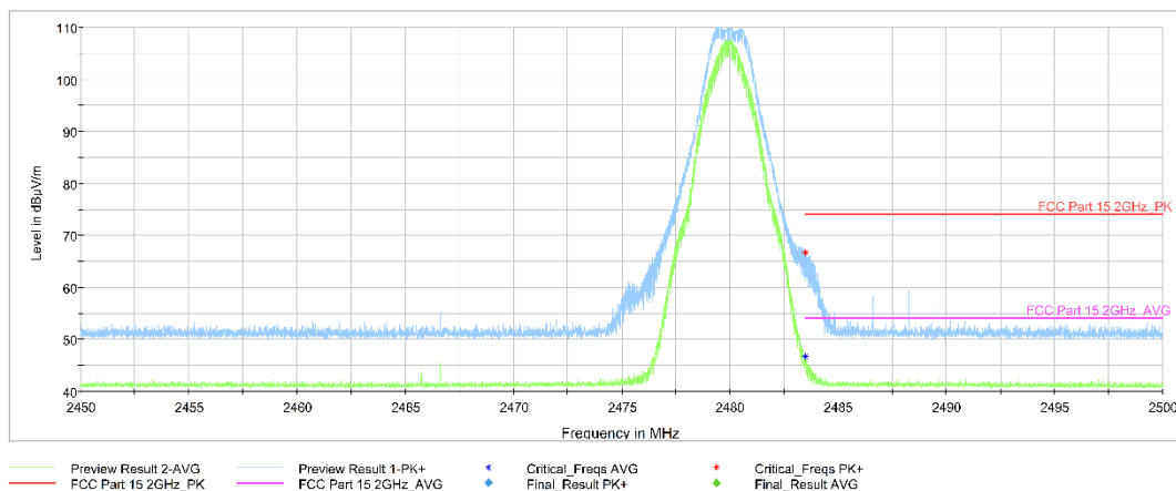
Fig.4. Frequency Band Edges: GFSK, 2480 MHz, Hopping Off , 2.45 GHz - 2.50GHz, SISO chain 0, unfolded
