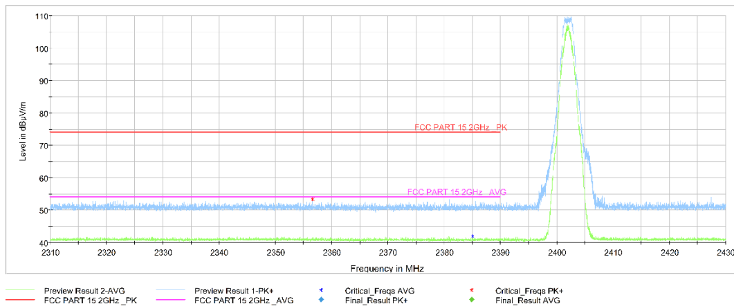
Fig.3. Frequency Band Edges: GFSK, 2402 MHz, Hopping Off, 2.31 GHz – 2.43GHz, SISO chain 0, unfolded
