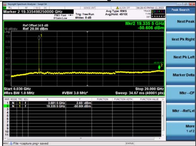
Band48C-30M-20G / 5MHz+20MHz / 1RB+1RB / QPSK / High CH
