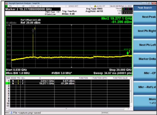
Band48C-30M-20G / 20MHz+5MHz / 1RB+1RB / QPSK / Mid CH
