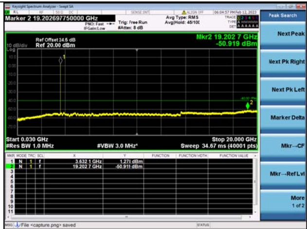
Band48C-30M-20G / 20MHz+5MHz / 1RB+1RB / QPSK / Mid CH
