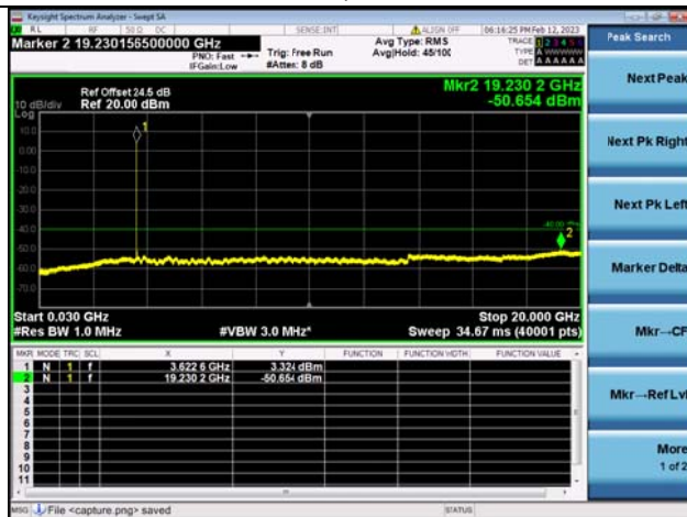
Band48C-30M-20G / 15MHz+20MHz / 1RB+1RB/ QPSK / Mid CH
