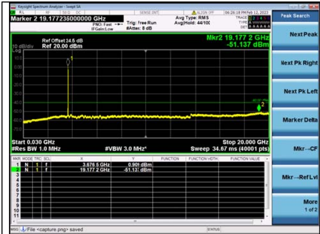
Band48C-30M-20G / 5MHz+20MHz / 1RB+1RB / QPSK / High CH
