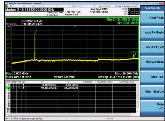
Band48C-30M-20G / 20MHz+20MHz /1RB+1RB/ QPSK / High CH
