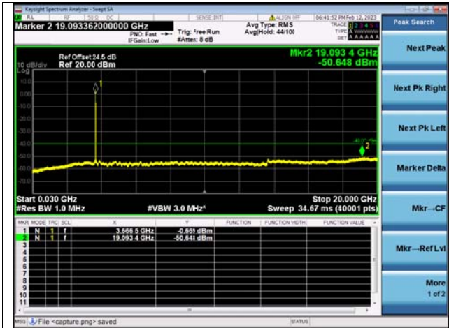
Band48C-30M-20G / 20MHz+15MHz /1RB+1RB/ QPSK / High CH
