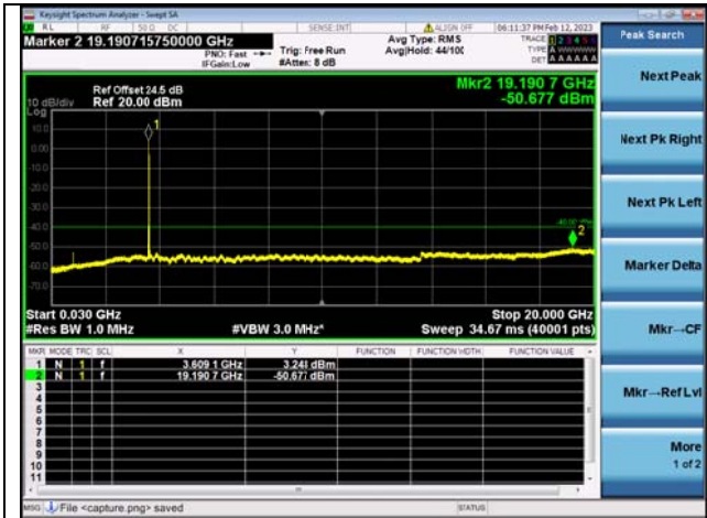
Band48C-30M-20G / 15MHz+20MHz / 1RB+1RB/ QPSK / Mid CH
