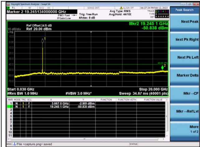
Band48C-30M-20G / 15MHz+20MHz /1RB+1RB/ QPSK / High CH
