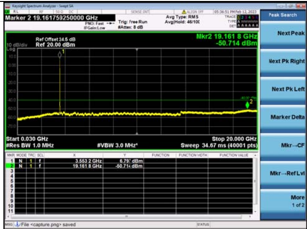
Band48C-30M-20G / 5MHz+20MHz / 25RB+100RB / QPSK / Low CH
