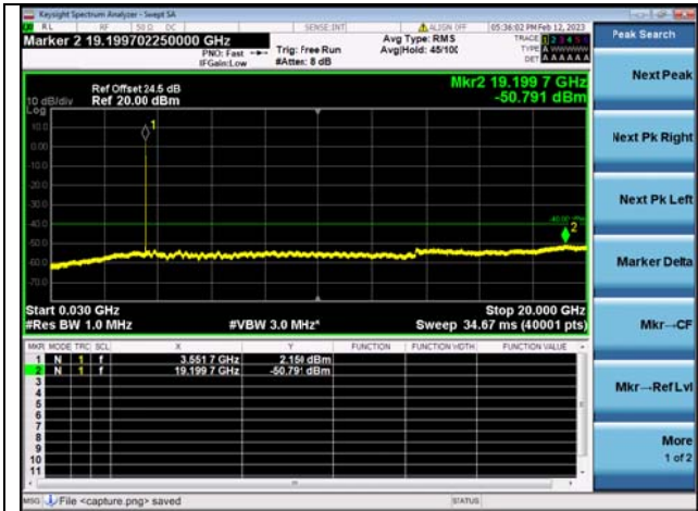
Band48C-30M-20G / 5MHz+20MHz / 1RB+1RB / QPSK / Low CH
