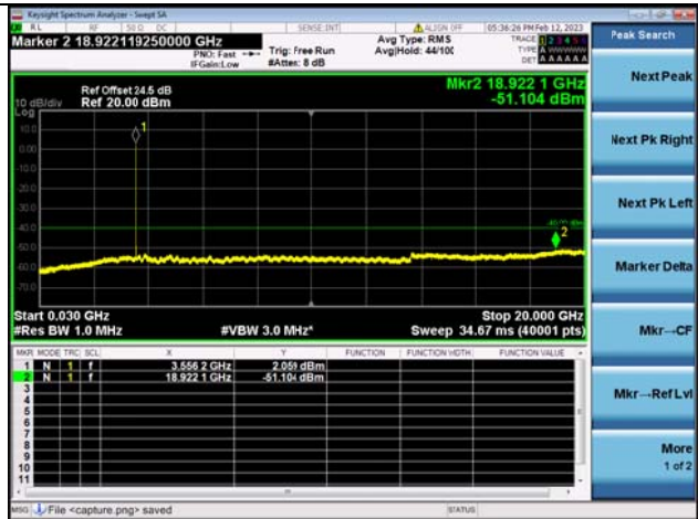
Band48C-30M-20G / 5MHz+20MHz / 1RB+1RB / QPSK / Low CH
