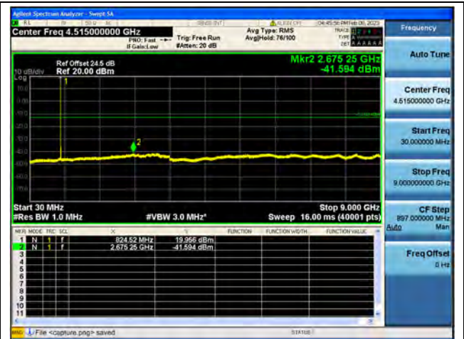
Band26Part22 / 5MHz / Low CH / 16QAM
