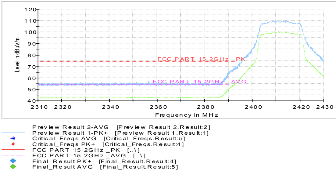
Fig.A.6.2.5 Transmitter Spurious Emission - Radiated (Power): 802.11n-HT20, ch1, 2.31 GHz - 2.43GHz
