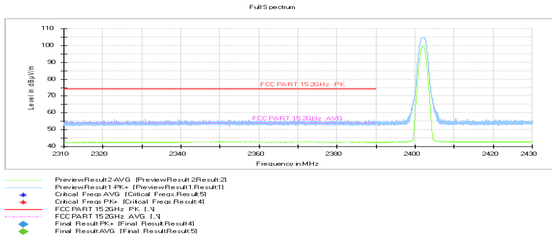
Fig.3. Frequency Band Edges: GFSK, 2402 MHz, 2.31 GHz – 2.43GHz
