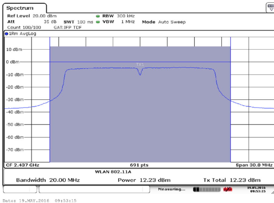
Fig.32 Maximum Average Output Power (802.11g, Ch 6,18Mbps)
