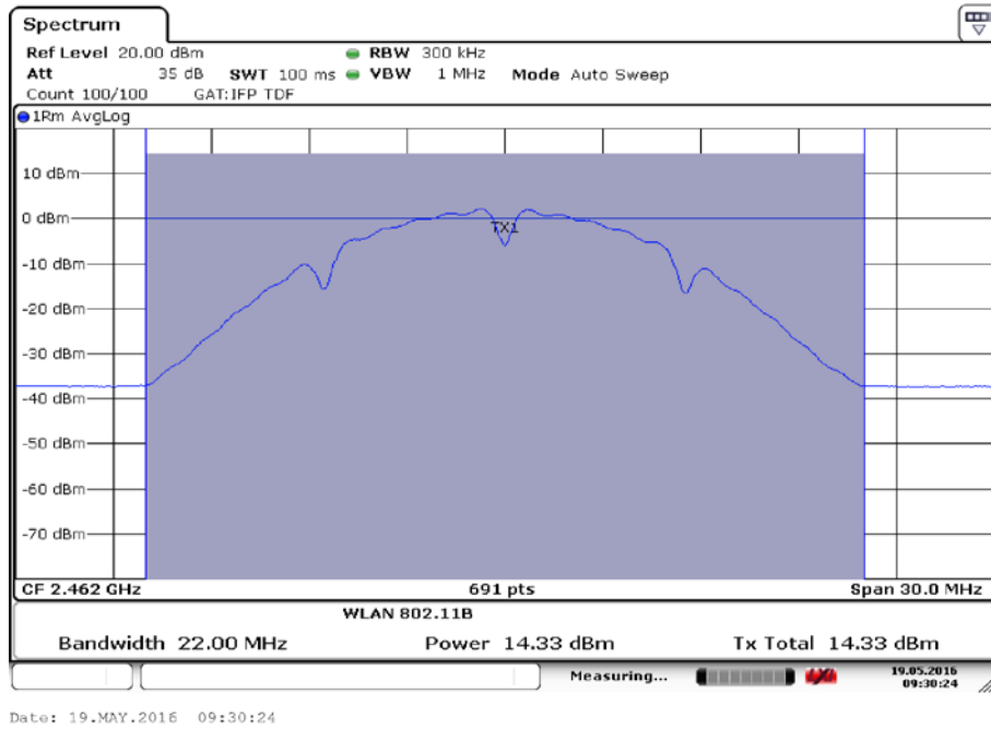
Fig.15 Maximum Average Output Power (802.11b, Ch 11,2Mbps)
