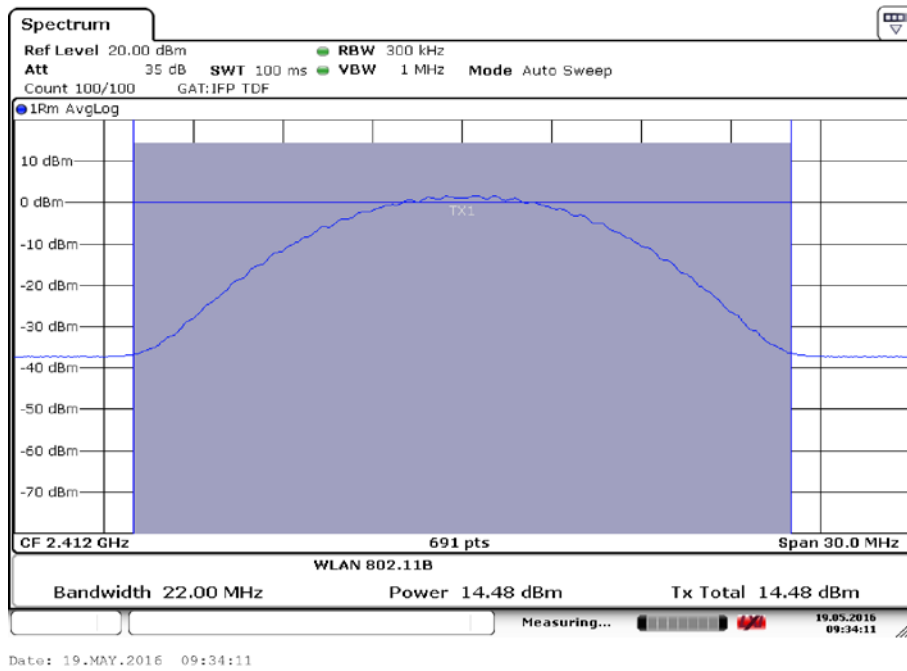
Fig.16 Maximum Average Output Power (802.11b, Ch 1,5Mbps)
