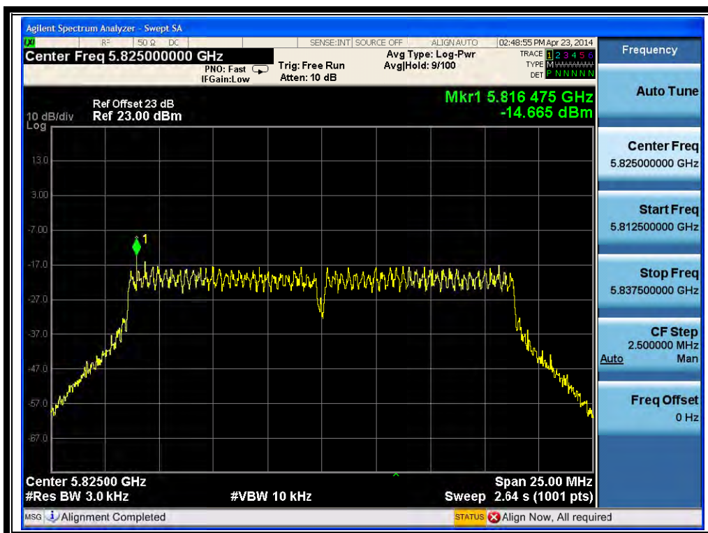
(Channel = 165 @ 802.11n-20MHz)
