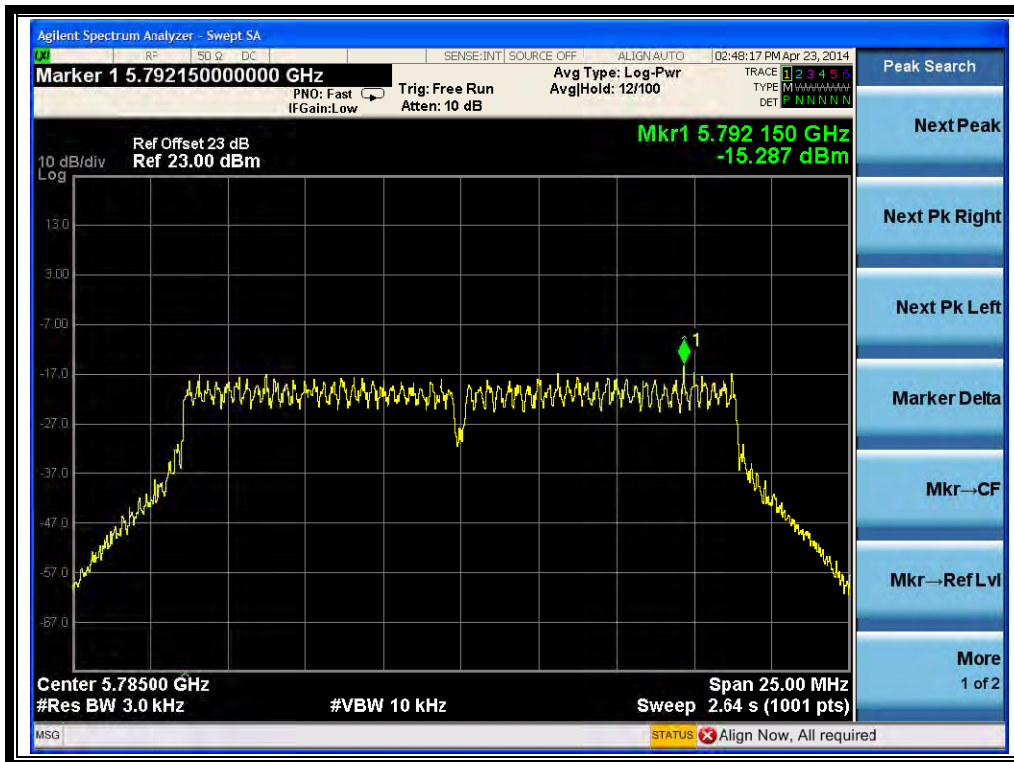
(Channel = 157 @ 802.11n-20MHz)
