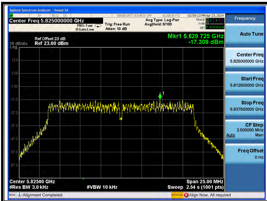
(Channel = 165 @ 802.11ac-20MHz)
