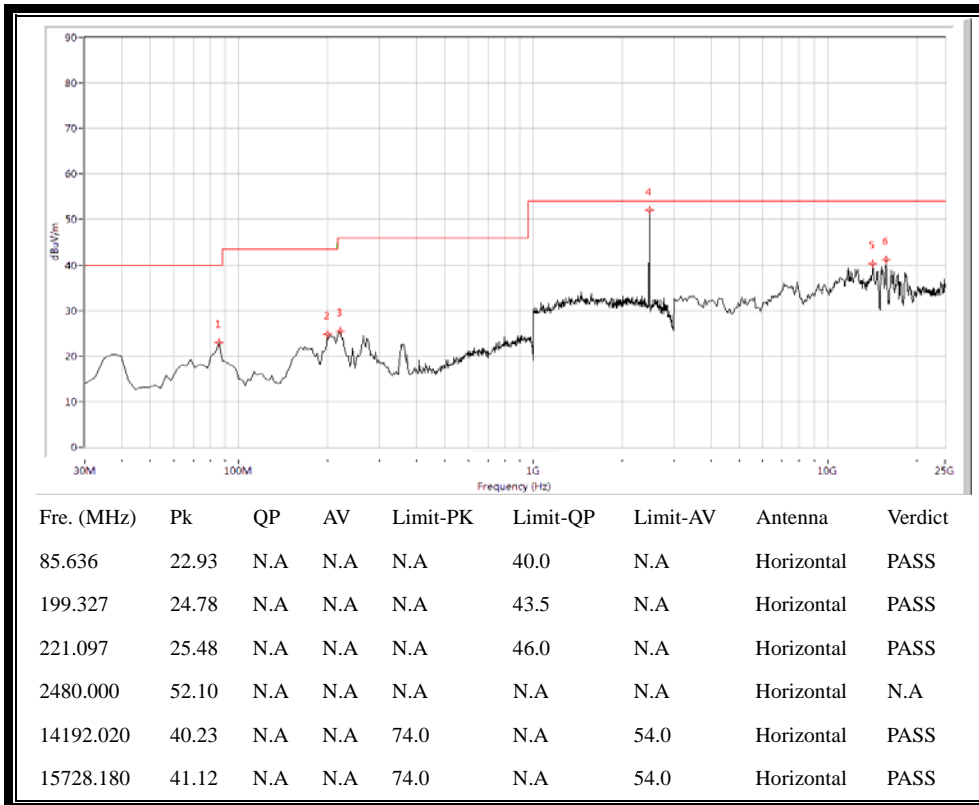
(Antenna Horizontal, 30MHz to 25GHz)
